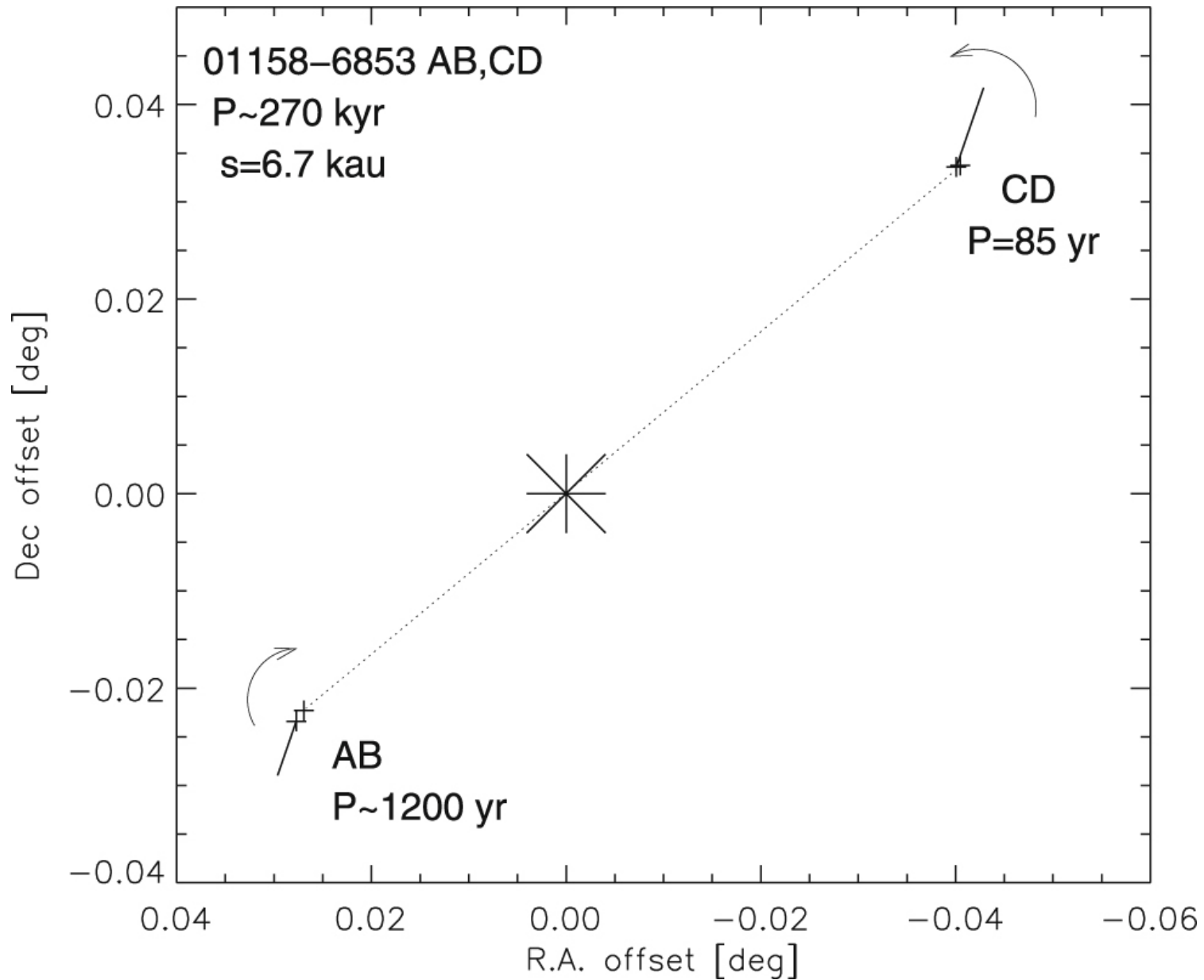
Figure 5. from Nearby Quintuple Systems Tucanae and Scorpii null 2020 AJ 159 265 doi:10.3847/1538-3881/ab8af1 https://dx.doi.org/10.3847/1538-3881/ab8af1 © 2020. The American Astronomical Society. All rights reserved.
