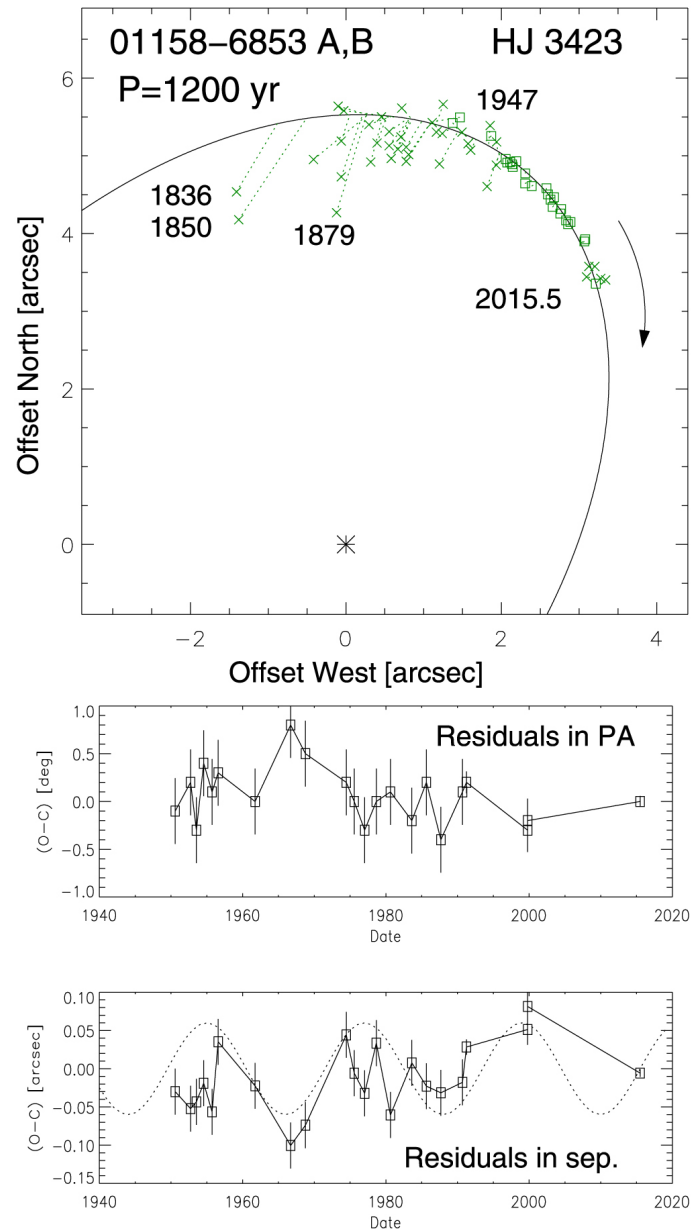
Figure 4. from Nearby Quintuple Systems Tucanae and Scorpii null 2020 AJ 159 265 doi:10.3847/1538-3881/ab8af1 https://dx.doi.org/10.3847/1538-3881/ab8af1 © 2020. The American Astronomical Society. All rights reserved.
