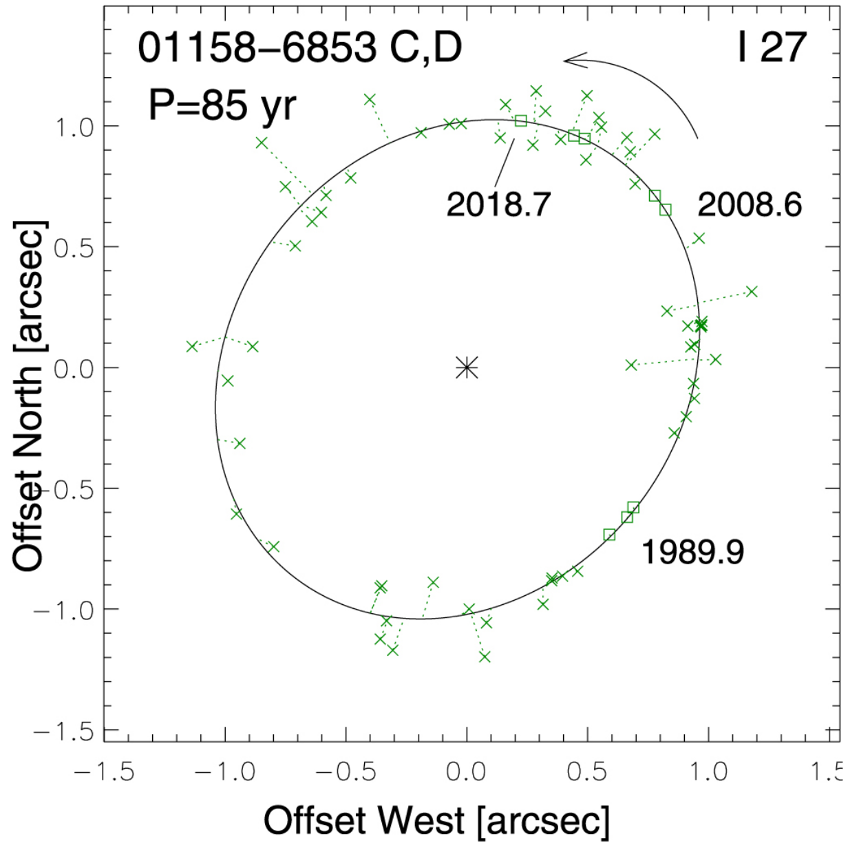
Figure 3. from Nearby Quintuple Systems Tucanae and Scorpii null 2020 AJ 159 265 doi:10.3847/1538-3881/ab8af1 https://dx.doi.org/10.3847/1538-3881/ab8af1 © 2020. The American Astronomical Society. All rights reserved.
