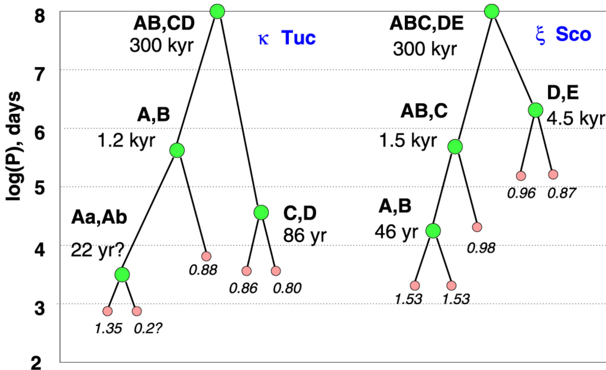
Figure 1. from Nearby Quintuple Systems Tucanae and Scorpii null 2020 AJ 159 265 doi:10.3847/1538-3881/ab8af1 https://dx.doi.org/10.3847/1538-3881/ab8af1 © 2020. The American Astronomical Society. All rights reserved.
