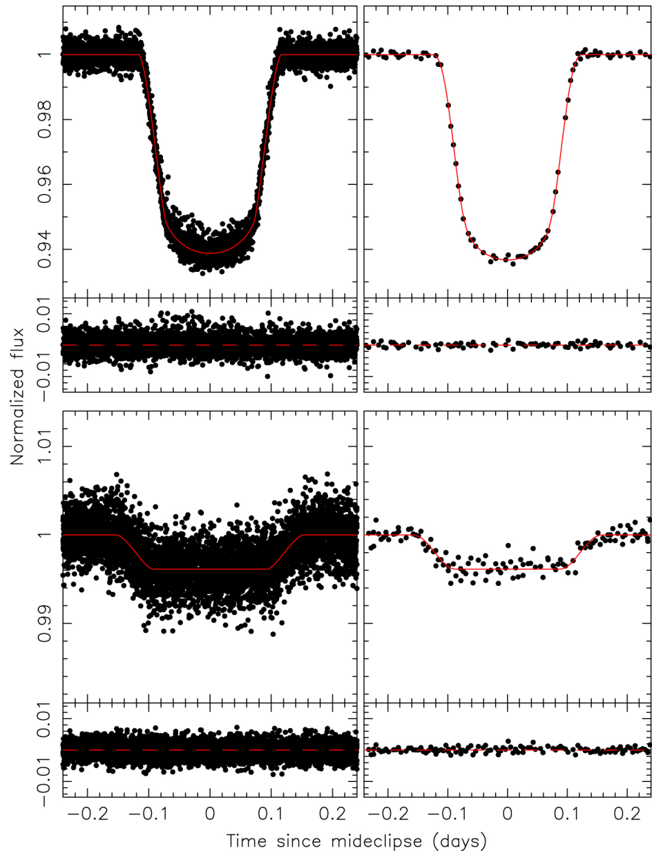
Figure 9. from TOI-1338: TESS' First Transiting Circumbinary Planet null 2020 AJ 159 253 doi:10.3847/1538-3881/ab8a48 https://dx.doi.org/10.3847/1538-3881/ab8a48 © 2020. The American Astronomical Society. All rights reserved.
