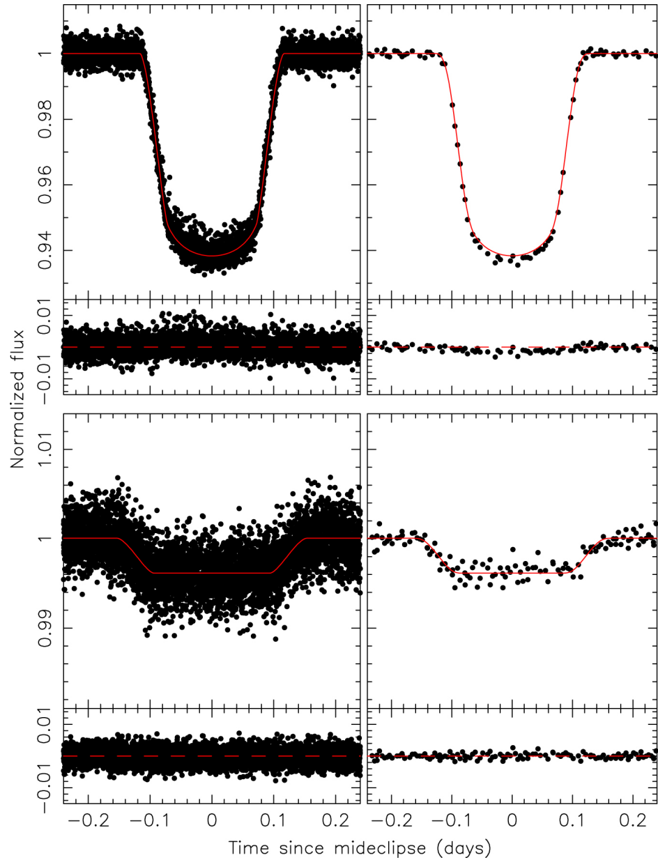
Figure 7. from TOI-1338: TESS' First Transiting Circumbinary Planet null 2020 AJ 159 253 doi:10.3847/1538-3881/ab8a48 https://dx.doi.org/10.3847/1538-3881/ab8a48 © 2020. The American Astronomical Society. All rights reserved.
