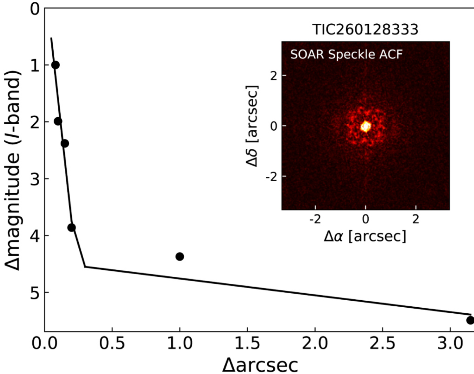
Figure 6. from TOI-1338: TESS' First Transiting Circumbinary Planet null 2020 AJ 159 253 doi:10.3847/1538-3881/ab8a48 https://dx.doi.org/10.3847/1538-3881/ab8a48 © 2020. The American Astronomical Society. All rights reserved.
