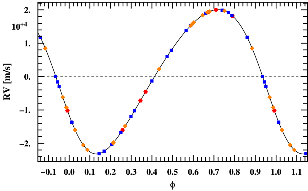
Figure 5. from TOI-1338: TESS' First Transiting Circumbinary Planet null 2020 AJ 159 253 doi:10.3847/1538-3881/ab8a48 https://dx.doi.org/10.3847/1538-3881/ab8a48 © 2020. The American Astronomical Society. All rights reserved.
