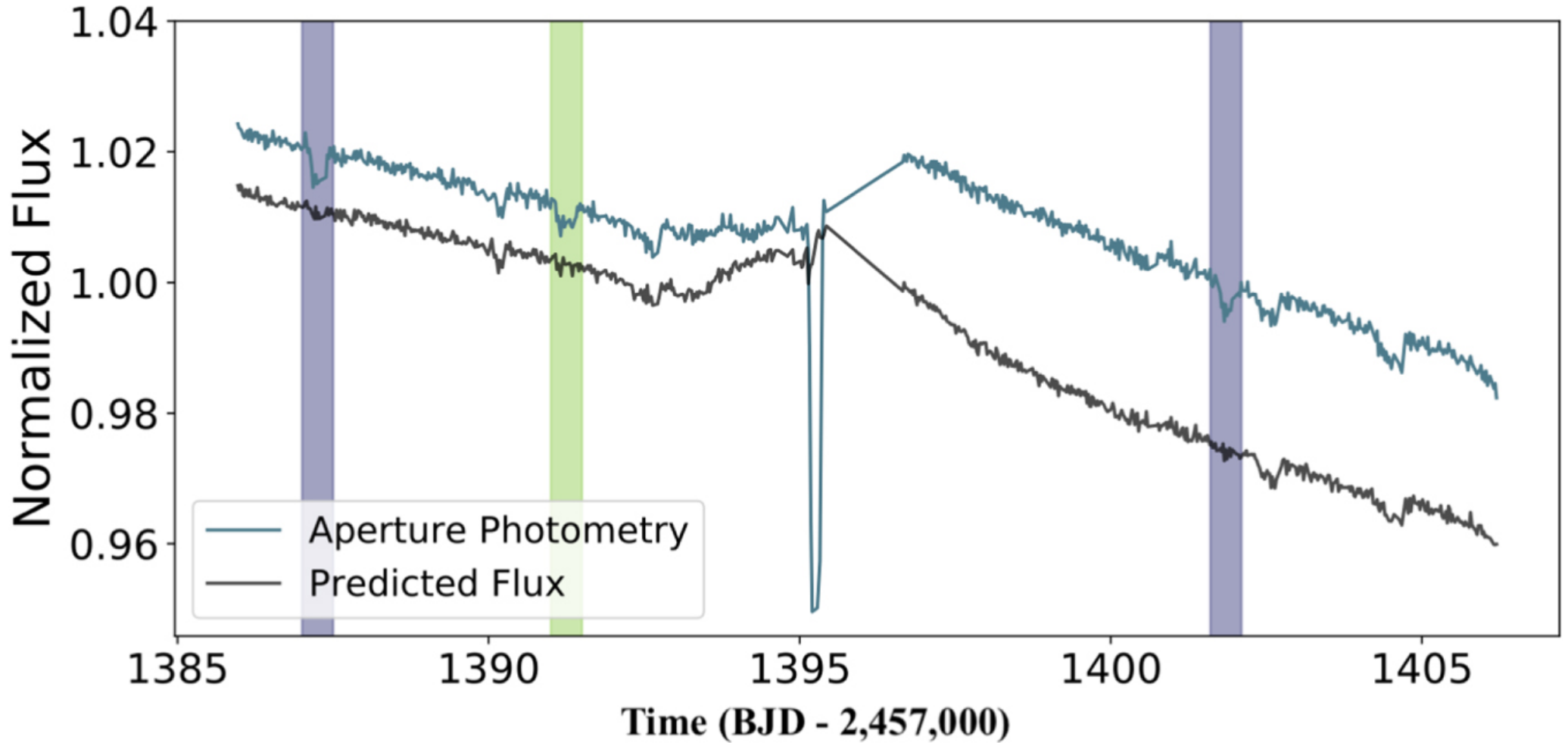
Figure 3. from TOI-1338: TESS' First Transiting Circumbinary Planet null 2020 AJ 159 253 doi:10.3847/1538-3881/ab8a48 https://dx.doi.org/10.3847/1538-3881/ab8a48 © 2020. The American Astronomical Society. All rights reserved.
