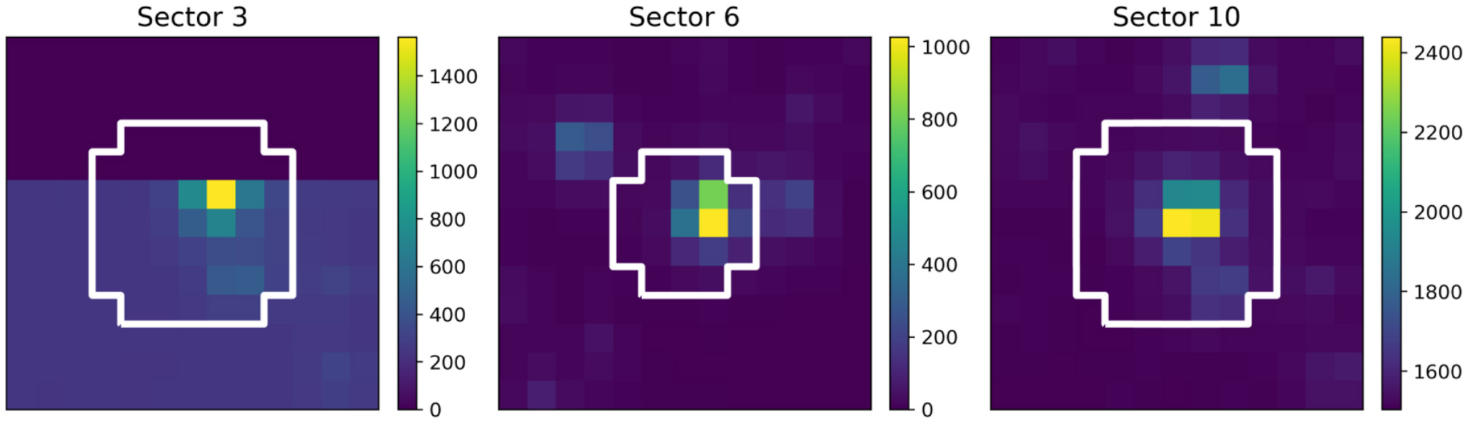
Figure 2. from TOI-1338: TESS' First Transiting Circumbinary Planet null 2020 AJ 159 253 doi:10.3847/1538-3881/ab8a48 https://dx.doi.org/10.3847/1538-3881/ab8a48 © 2020. The American Astronomical Society. All rights reserved.
