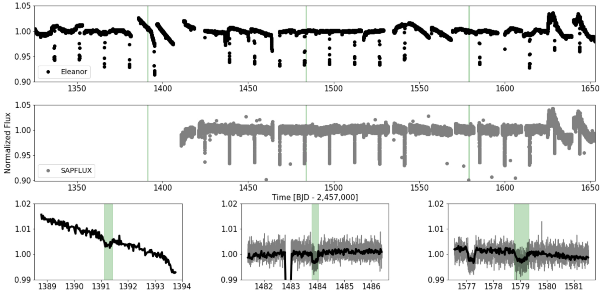
Figure 1. from TOI-1338: TESS' First Transiting Circumbinary Planet null 2020 AJ 159 253 doi:10.3847/1538-3881/ab8a48 https://dx.doi.org/10.3847/1538-3881/ab8a48 © 2020. The American Astronomical Society. All rights reserved.
