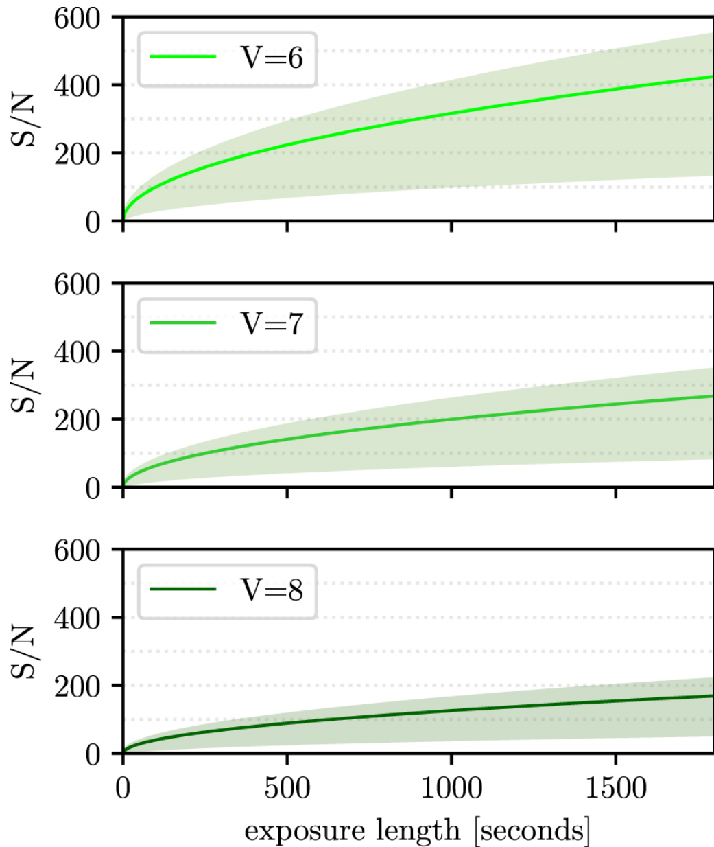
Figure 6. from Performance Verification of the EXtreme PREcision Spectrograph null 2020 AJ 159 238 doi:10.3847/1538-3881/ab811d https://dx.doi.org/10.3847/1538-3881/ab811d © 2020. The American Astronomical Society. All rights reserved.
