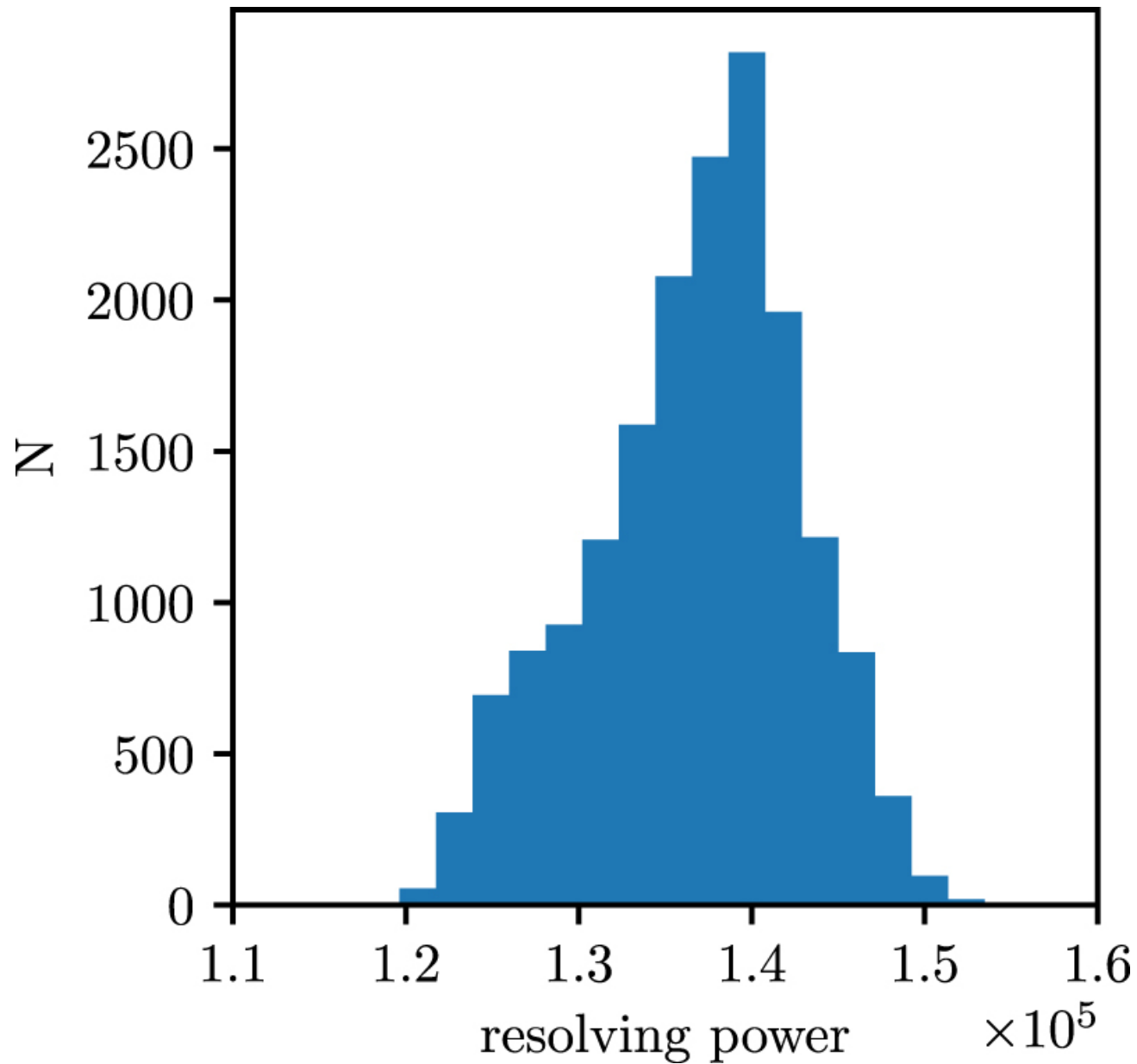
Figure 4. from Performance Verification of the EXtreme PREcision Spectrograph null 2020 AJ 159 238 doi:10.3847/1538-3881/ab811d https://dx.doi.org/10.3847/1538-3881/ab811d © 2020. The American Astronomical Society. All rights reserved.
