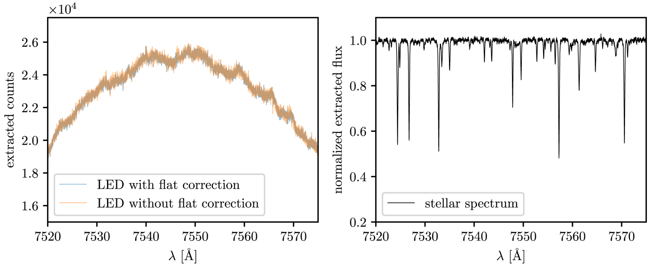
Figure 25. from Performance Verification of the EXtreme PREcision Spectrograph null 2020 AJ 159 238 doi:10.3847/1538-3881/ab811d https://dx.doi.org/10.3847/1538-3881/ab811d © 2020. The American Astronomical Society. All rights reserved.
