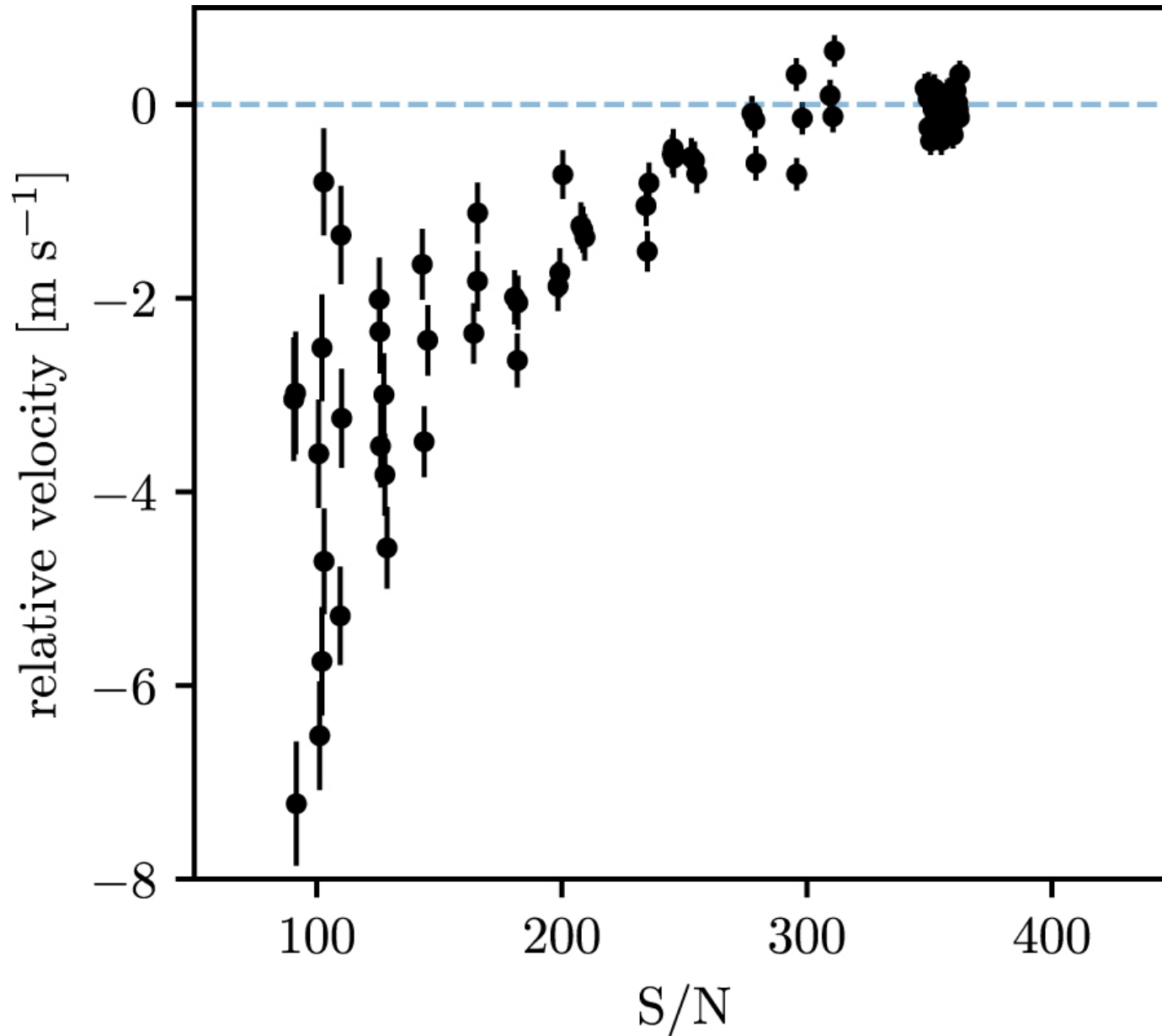
Figure 24. from Performance Verification of the EXtreme PREcision Spectrograph null 2020 AJ 159 238 doi:10.3847/1538-3881/ab811d https://dx.doi.org/10.3847/1538-3881/ab811d © 2020. The American Astronomical Society. All rights reserved.
