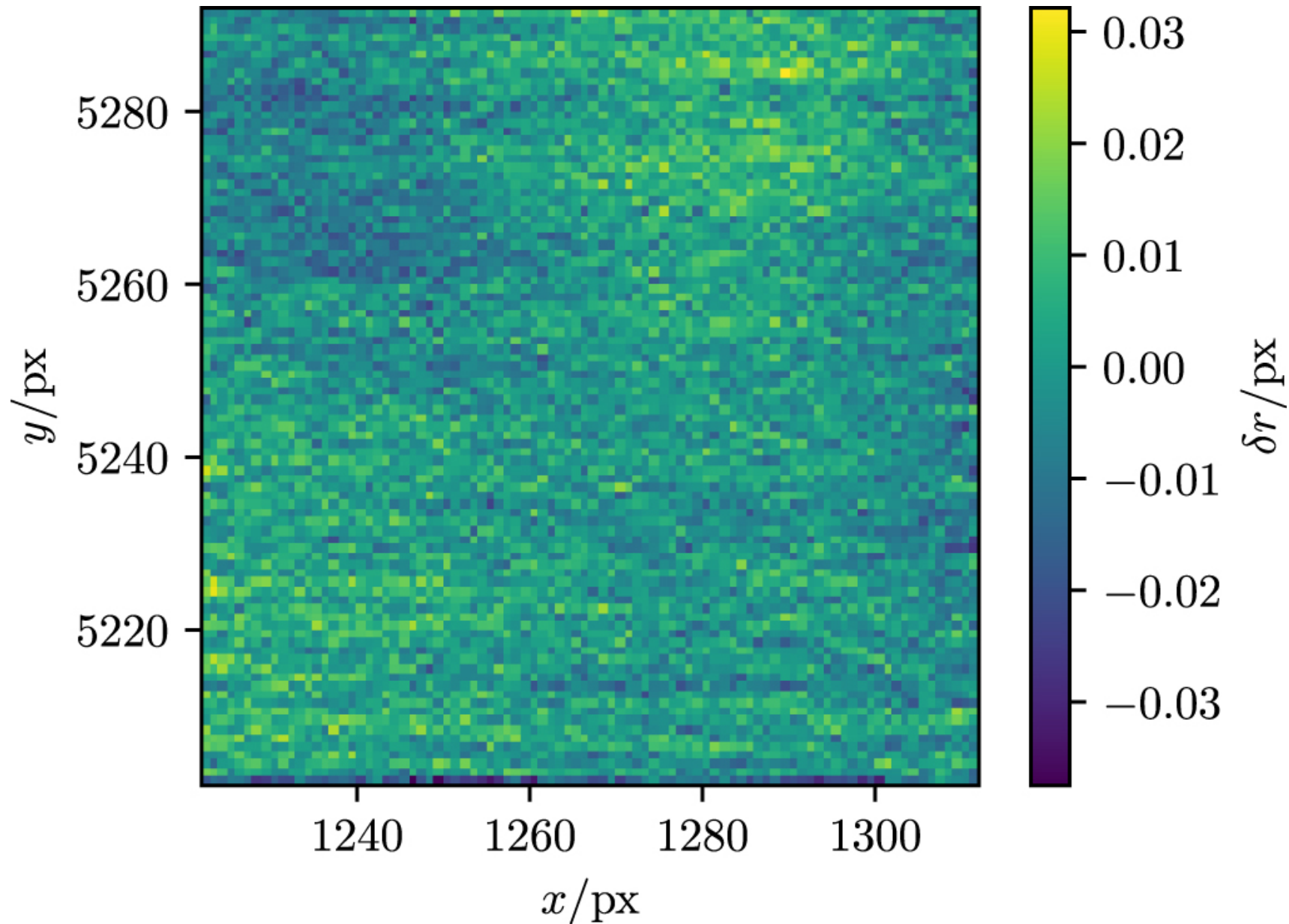
Figure 22. from Performance Verification of the EXtreme PREcision Spectrograph null 2020 AJ 159 238 doi:10.3847/1538-3881/ab811d https://dx.doi.org/10.3847/1538-3881/ab811d © 2020. The American Astronomical Society. All rights reserved.
