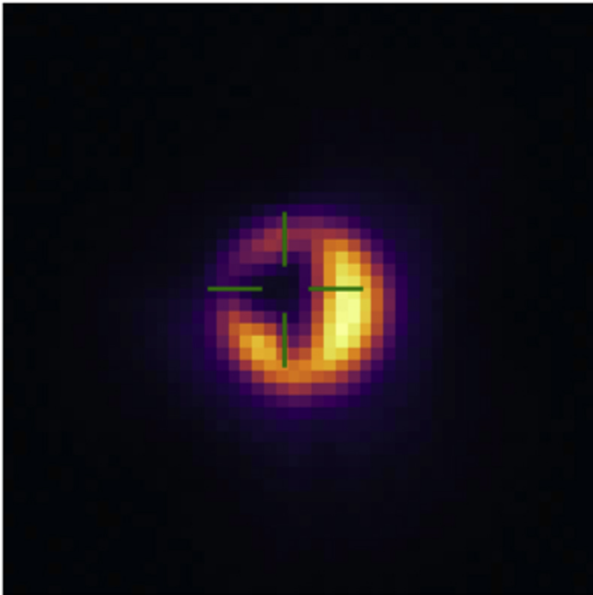
Figure 2. from Performance Verification of the EXtreme PREcision Spectrograph null 2020 AJ 159 238 doi:10.3847/1538-3881/ab811d https://dx.doi.org/10.3847/1538-3881/ab811d © 2020. The American Astronomical Society. All rights reserved.
