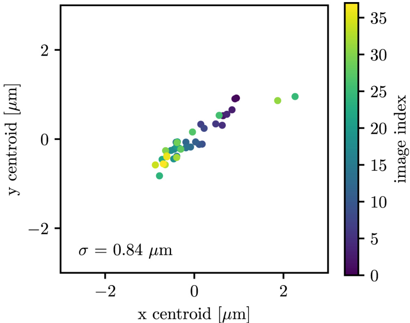
Figure 17. from Performance Verification of the EXtreme PREcision Spectrograph null 2020 AJ 159 238 doi:10.3847/1538-3881/ab811d https://dx.doi.org/10.3847/1538-3881/ab811d © 2020. The American Astronomical Society. All rights reserved.
