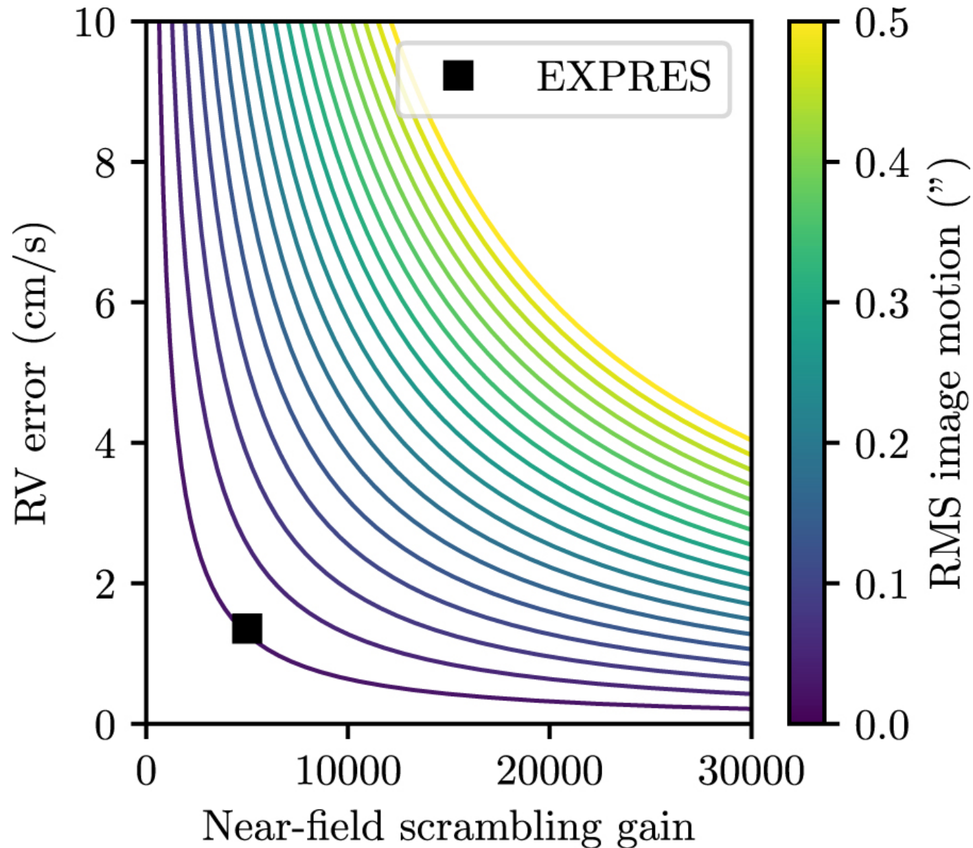
Figure 15. from Performance Verification of the EXtreme PREcision Spectrograph null 2020 AJ 159 238 doi:10.3847/1538-3881/ab811d https://dx.doi.org/10.3847/1538-3881/ab811d © 2020. The American Astronomical Society. All rights reserved.
