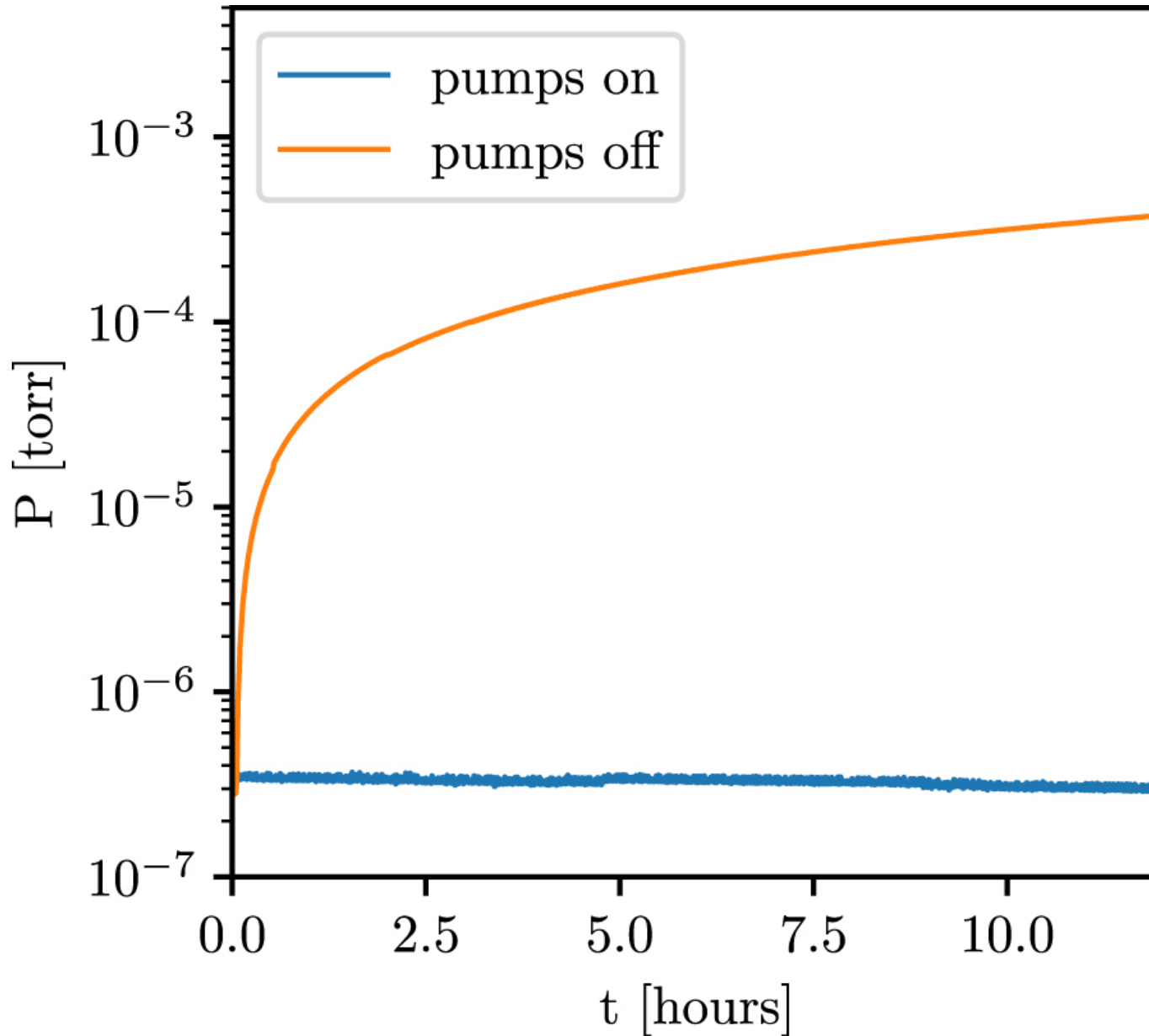
Figure 10. from Performance Verification of the EXtreme PREcision Spectrograph null 2020 AJ 159 238 doi:10.3847/1538-3881/ab811d https://dx.doi.org/10.3847/1538-3881/ab811d © 2020. The American Astronomical Society. All rights reserved.
