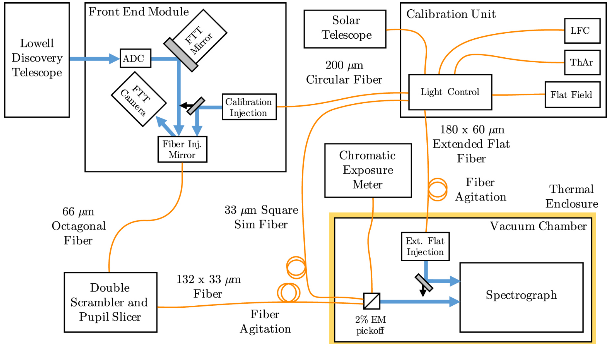
Figure 1. from Performance Verification of the EXtreme PREcision Spectrograph null 2020 AJ 159 238 doi:10.3847/1538-3881/ab811d https://dx.doi.org/10.3847/1538-3881/ab811d © 2020. The American Astronomical Society. All rights reserved.
