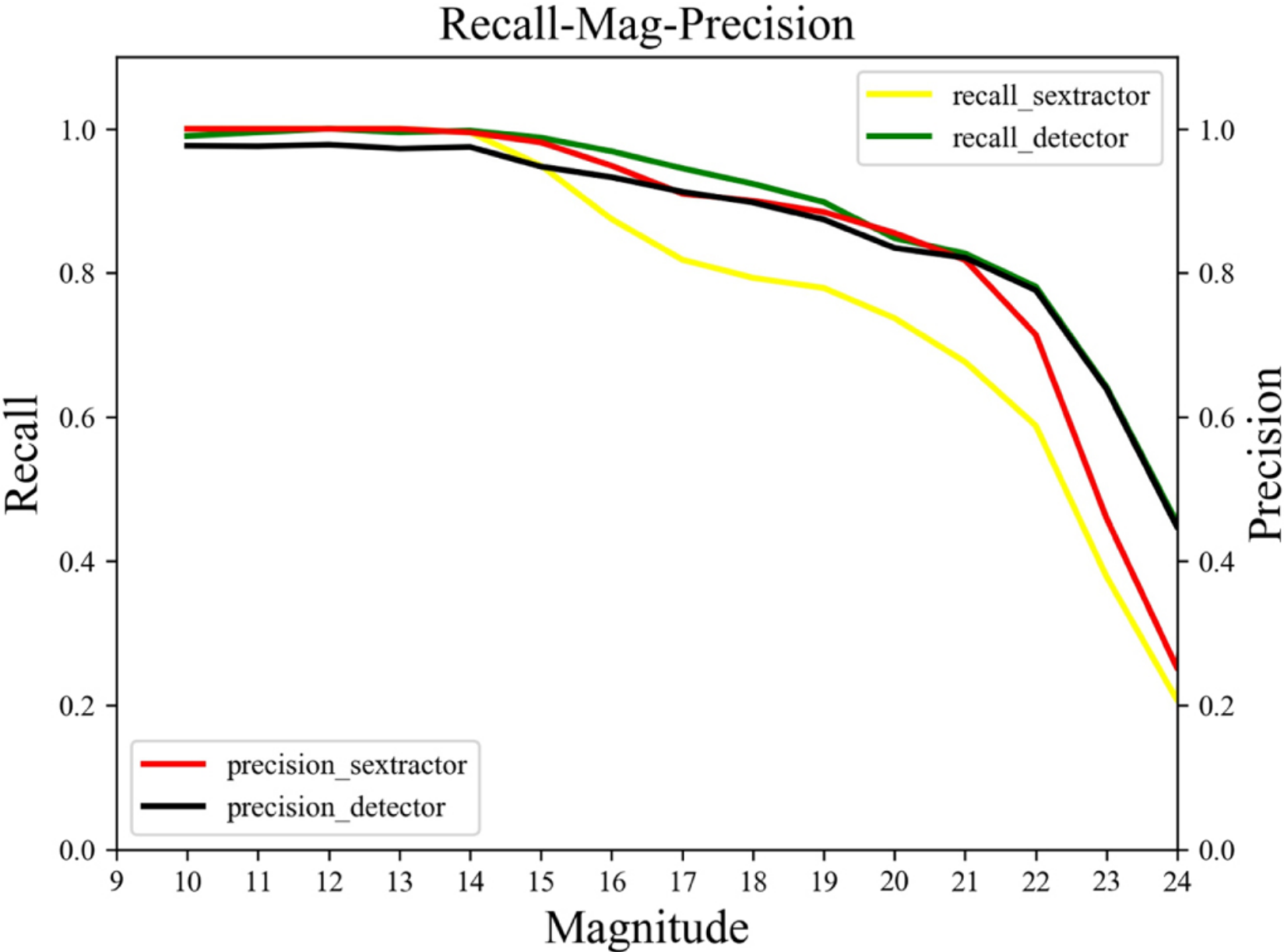
Figure 8. from Detection and Classification of Astronomical Targets with Deep Neural Networks in Wide-field Small Aperture Telescopes null 2020 AJ 159 212 doi:10.3847/1538-3881/ab800a https://dx.doi.org/10.3847/1538-3881/ab800a © 2020. The American Astronomical Society. All rights reserved.
