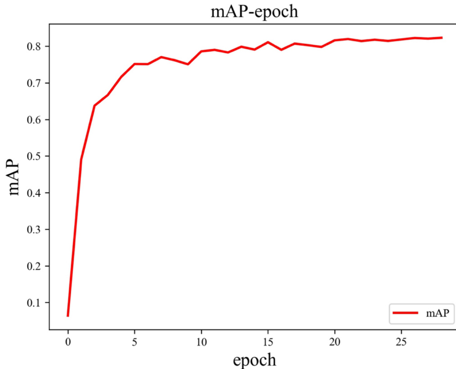
Figure 5. from Detection and Classification of Astronomical Targets with Deep Neural Networks in Wide-field Small Aperture Telescopes null 2020 AJ 159 212 doi:10.3847/1538-3881/ab800a https://dx.doi.org/10.3847/1538-3881/ab800a © 2020. The American Astronomical Society. All rights reserved.
