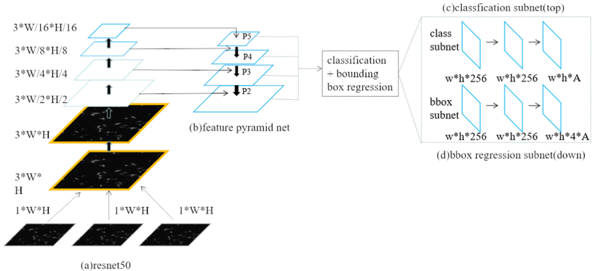
Figure 1. from Detection and Classification of Astronomical Targets with Deep Neural Networks in Wide-field Small Aperture Telescopes null 2020 AJ 159 212 doi:10.3847/1538-3881/ab800a https://dx.doi.org/10.3847/1538-3881/ab800a © 2020. The American Astronomical Society. All rights reserved.
