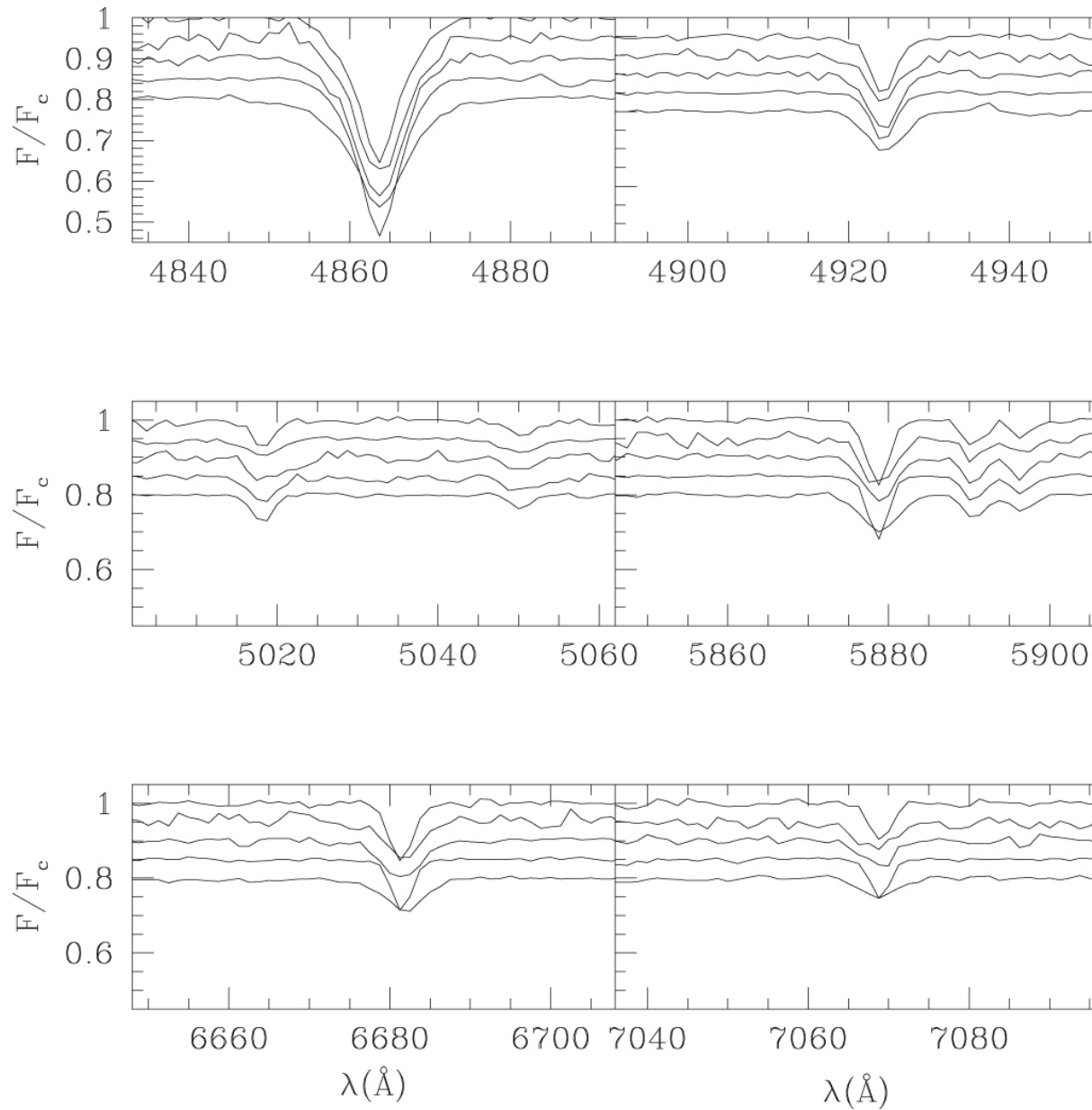
Figure 8. from MUSE Observations of NGC330 in the Small Magellanic Cloud: Helium Abundance of Bright Main-sequence Stars null 2020 AJ 159 152 doi:10.3847/1538-3881/ab7334 https://dx.doi.org/10.3847/1538-3881/ab7334
