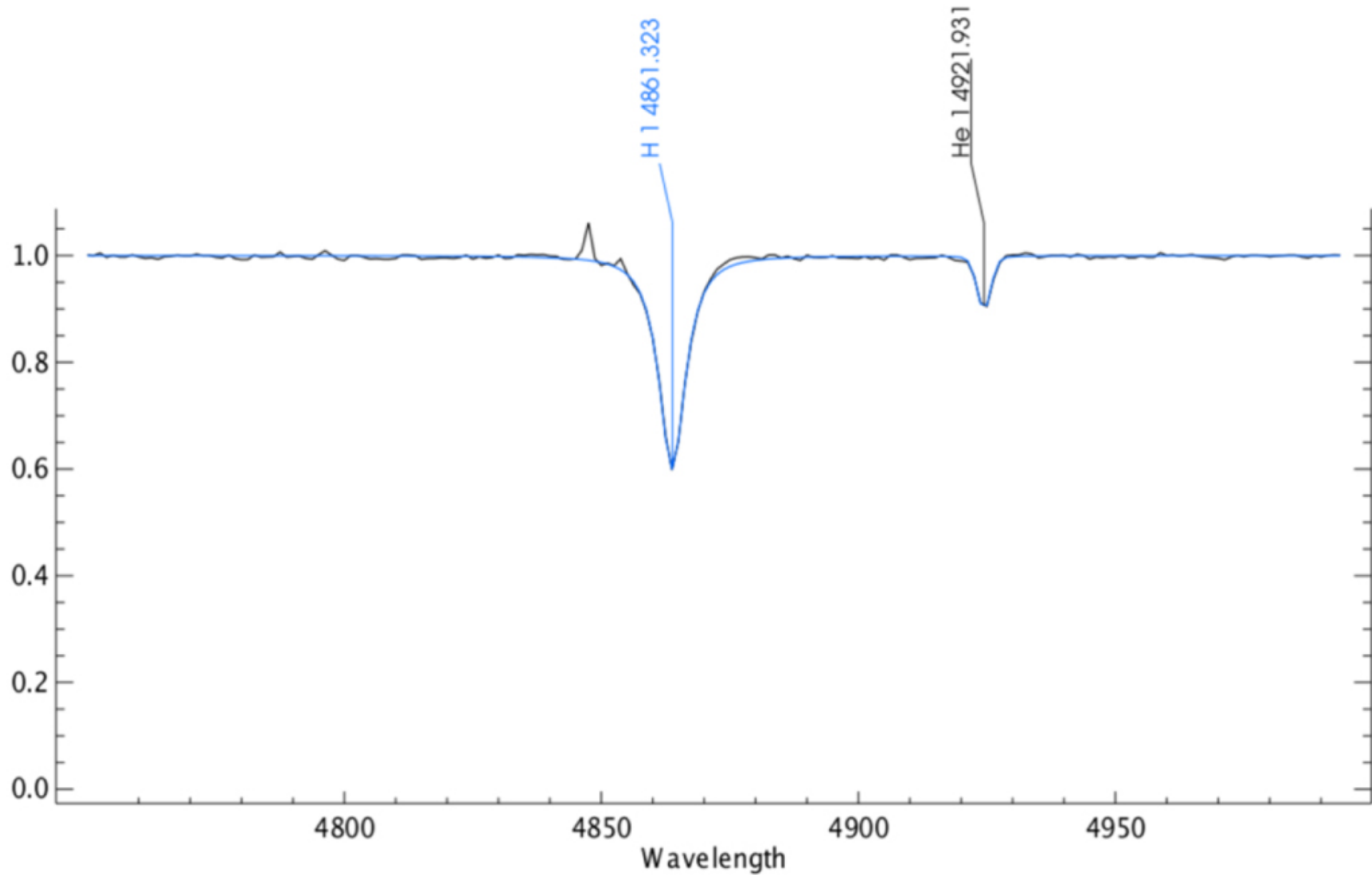
Figure 6. from MUSE Observations of NGC330 in the Small Magellanic Cloud: Helium Abundance of Bright Main-sequence Stars null 2020 AJ 159 152 doi:10.3847/1538-3881/ab7334 https://dx.doi.org/10.3847/1538-3881/ab7334 © 2020. The American Astronomical Society. All rights reserved.
