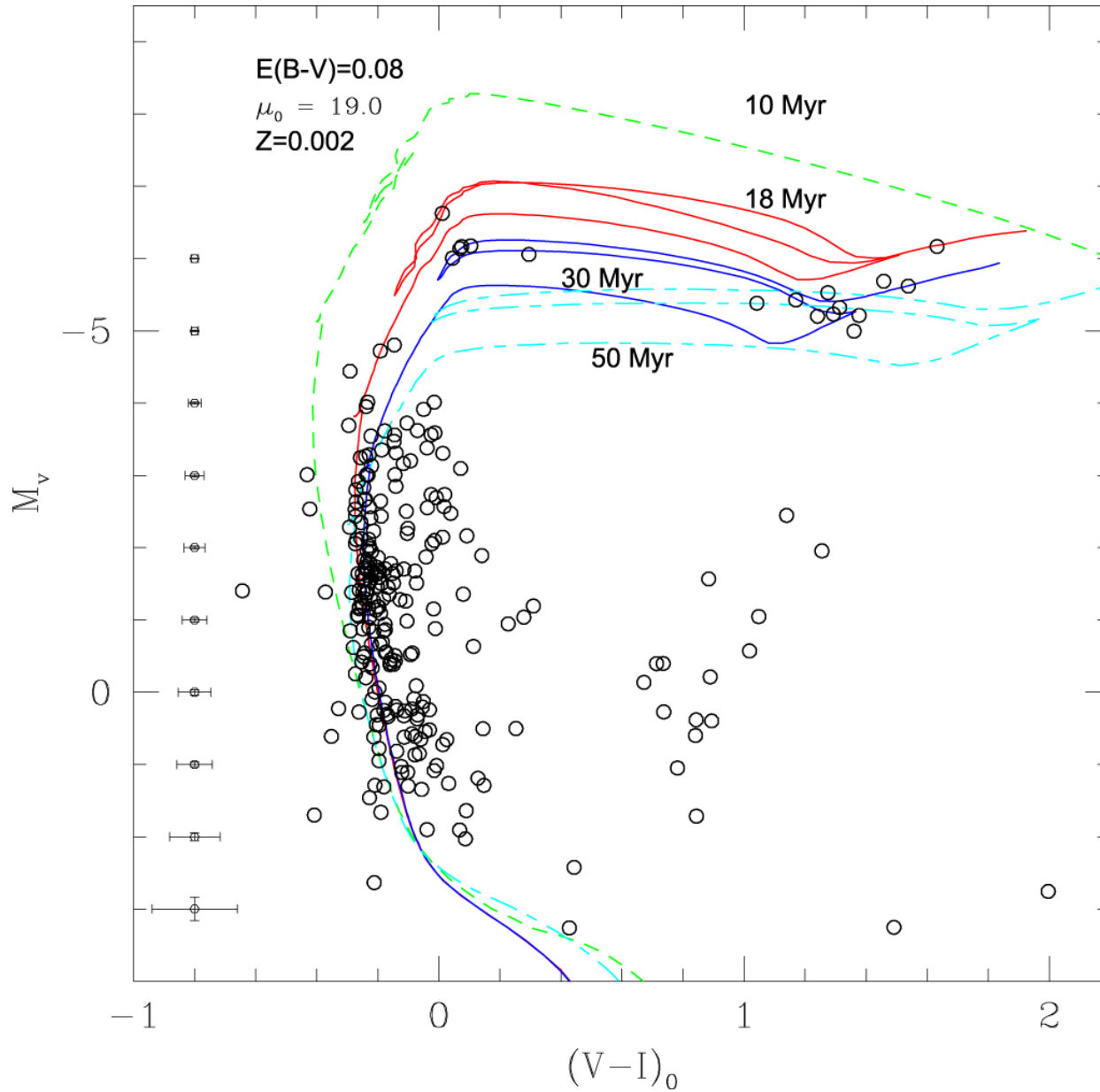
Figure 4. from MUSE Observations of NGC330 in the Small Magellanic Cloud: Helium Abundance of Bright Main-sequence Stars null 2020 AJ 159 152 doi:10.3847/1538-3881/ab7334 https://dx.doi.org/10.3847/1538-3881/ab7334 © 2020. The American Astronomical Society. All rights reserved.
