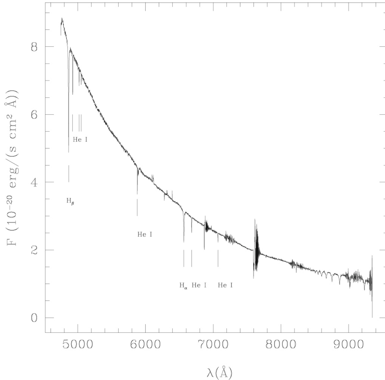
Figure 3. from MUSE Observations of NGC330 in the Small Magellanic Cloud: Helium Abundance of Bright Main-sequence Stars null 2020 AJ 159 152 doi:10.3847/1538-3881/ab7334 https://dx.doi.org/10.3847/1538-3881/ab7334 © 2020. The American Astronomical Society. All rights reserved.
