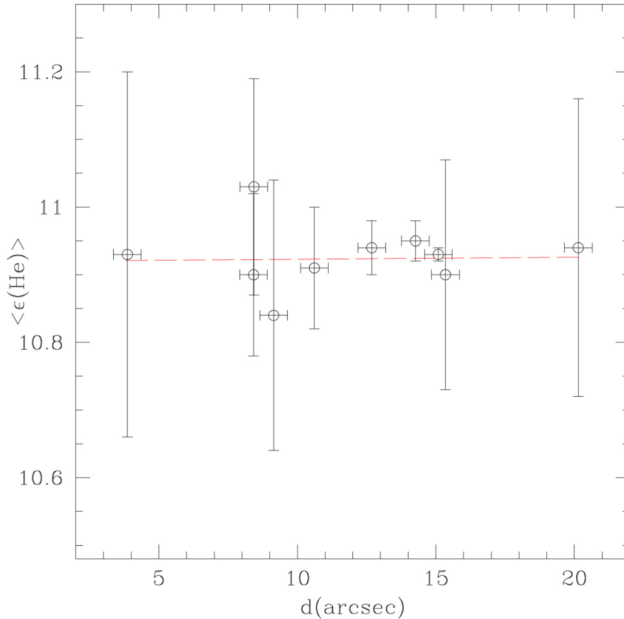
Figure 14. from MUSE Observations of NGC330 in the Small Magellanic Cloud: Helium Abundance of Bright Main-sequence Stars null 2020 AJ 159 152 doi:10.3847/1538-3881/ab7334 https://dx.doi.org/10.3847/1538-3881/ab7334 © 2020. The American Astronomical Society. All rights reserved.
