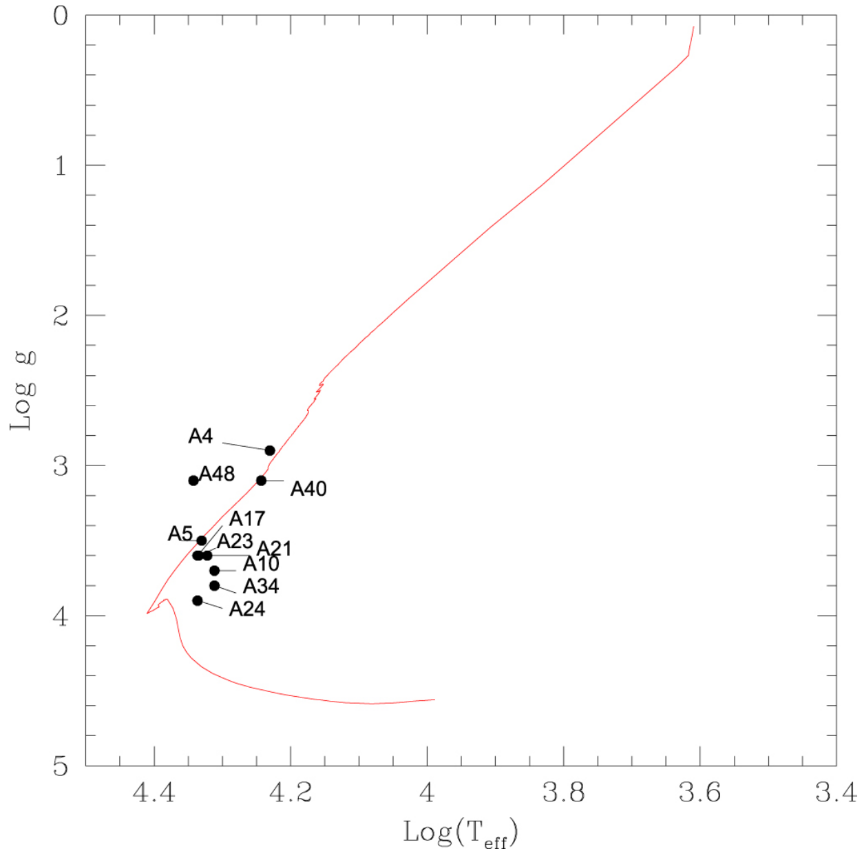
Figure 13. from MUSE Observations of NGC330 in the Small Magellanic Cloud: Helium Abundance of Bright Main-sequence Stars null 2020 AJ 159 152 doi:10.3847/1538-3881/ab7334 https://dx.doi.org/10.3847/1538-3881/ab7334 © 2020. The American Astronomical Society. All rights reserved.
