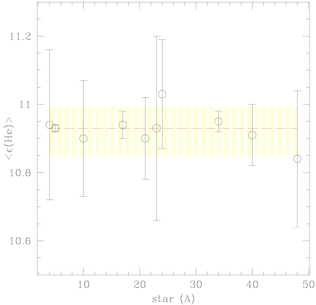
Figure 11. from MUSE Observations of NGC330 in the Small Magellanic Cloud: Helium Abundance of Bright Main-sequence Stars null 2020 AJ 159 152 doi:10.3847/1538-3881/ab7334 https://dx.doi.org/10.3847/1538-3881/ab7334 © 2020. The American Astronomical Society. All rights reserved.
