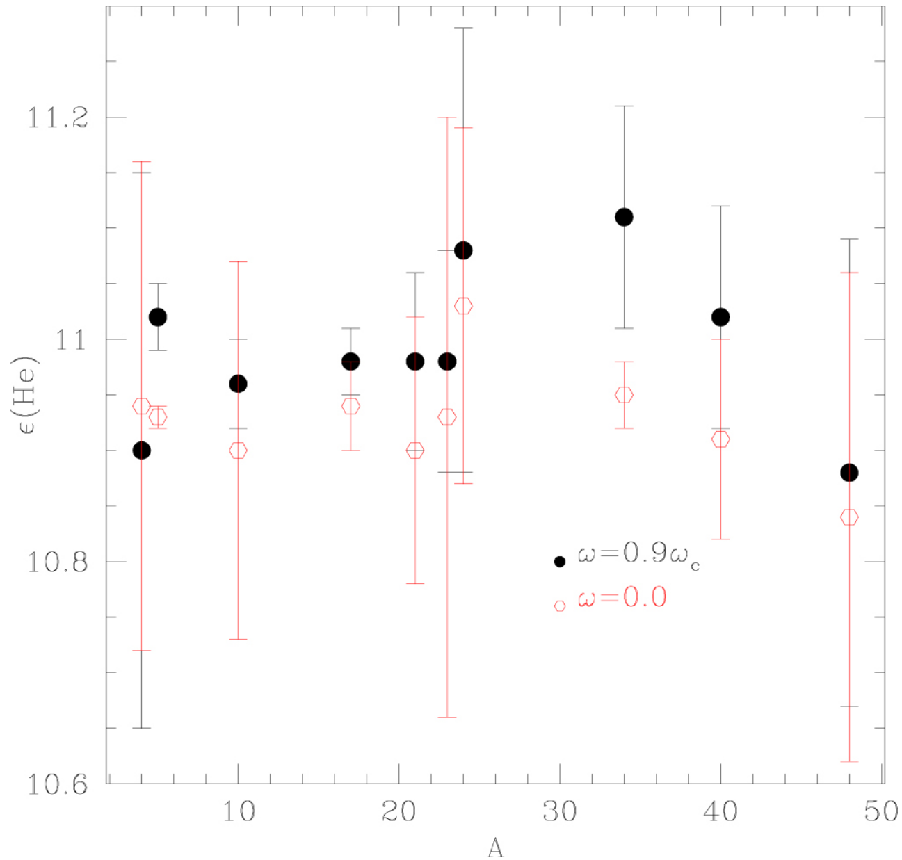
Figure 10. from MUSE Observations of NGC330 in the Small Magellanic Cloud: Helium Abundance of Bright Main-sequence Stars null 2020 AJ 159 152 doi:10.3847/1538-3881/ab7334 https://dx.doi.org/10.3847/1538-3881/ab7334 © 2020. The American Astronomical Society. All rights reserved.
