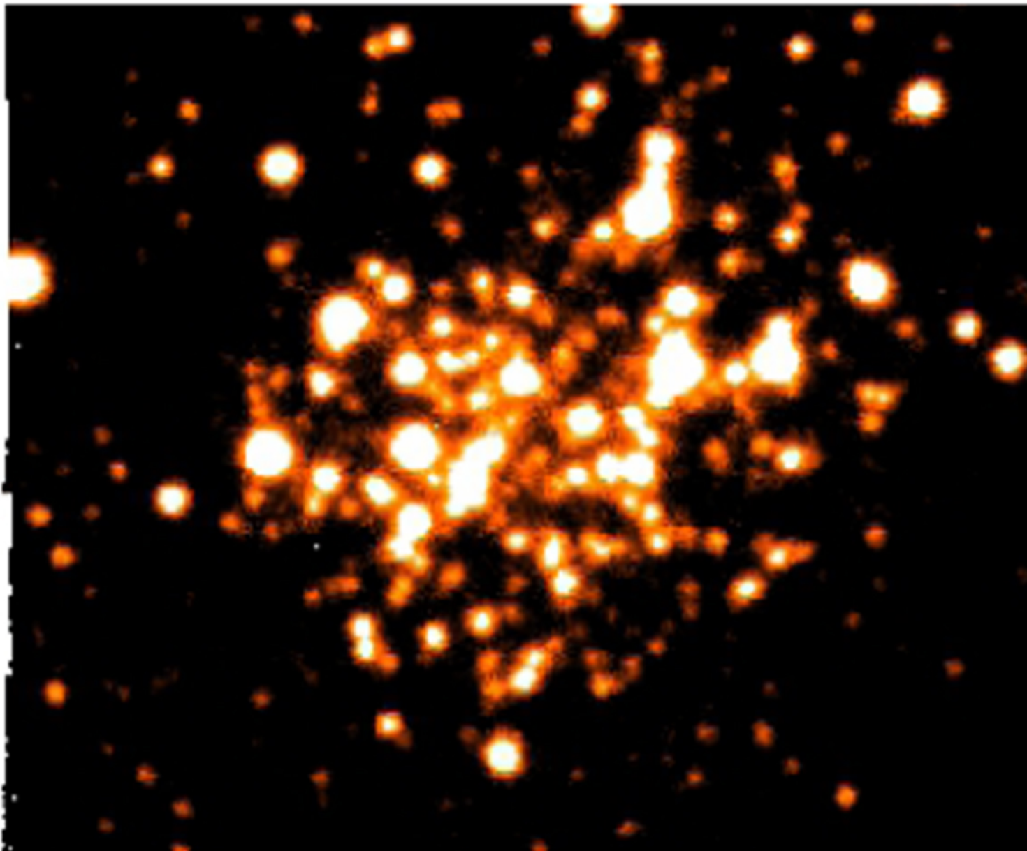
Figure 1. from MUSE Observations of NGC330 in the Small Magellanic Cloud: Helium Abundance of Bright Main-sequence Stars null 2020 AJ 159 152 doi:10.3847/1538-3881/ab7334 https://dx.doi.org/10.3847/1538-3881/ab7334 © 2020. The American Astronomical Society. All rights reserved.
