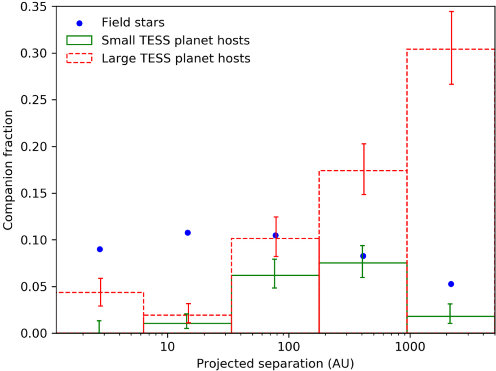
Figure 8. from SOAR TESS Survey. I. Sculpting of TESS Planetary Systems by Stellar Companions null 2020 AJ 159 19 doi:10.3847/1538-3881/ab55e9 https://dx.doi.org/10.3847/1538-3881/ab55e9 © 2019. The American Astronomical Society. All rights reserved.
