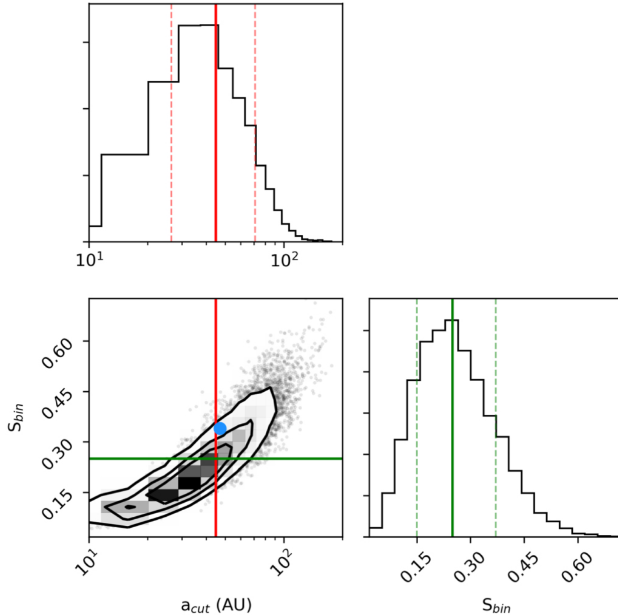
Figure 7. from SOAR TESS Survey. I. Sculpting of TESS Planetary Systems by Stellar Companions null 2020 AJ 159 19 doi:10.3847/1538-3881/ab55e9 https://dx.doi.org/10.3847/1538-3881/ab55e9 © 2019. The American Astronomical Society. All rights reserved.
