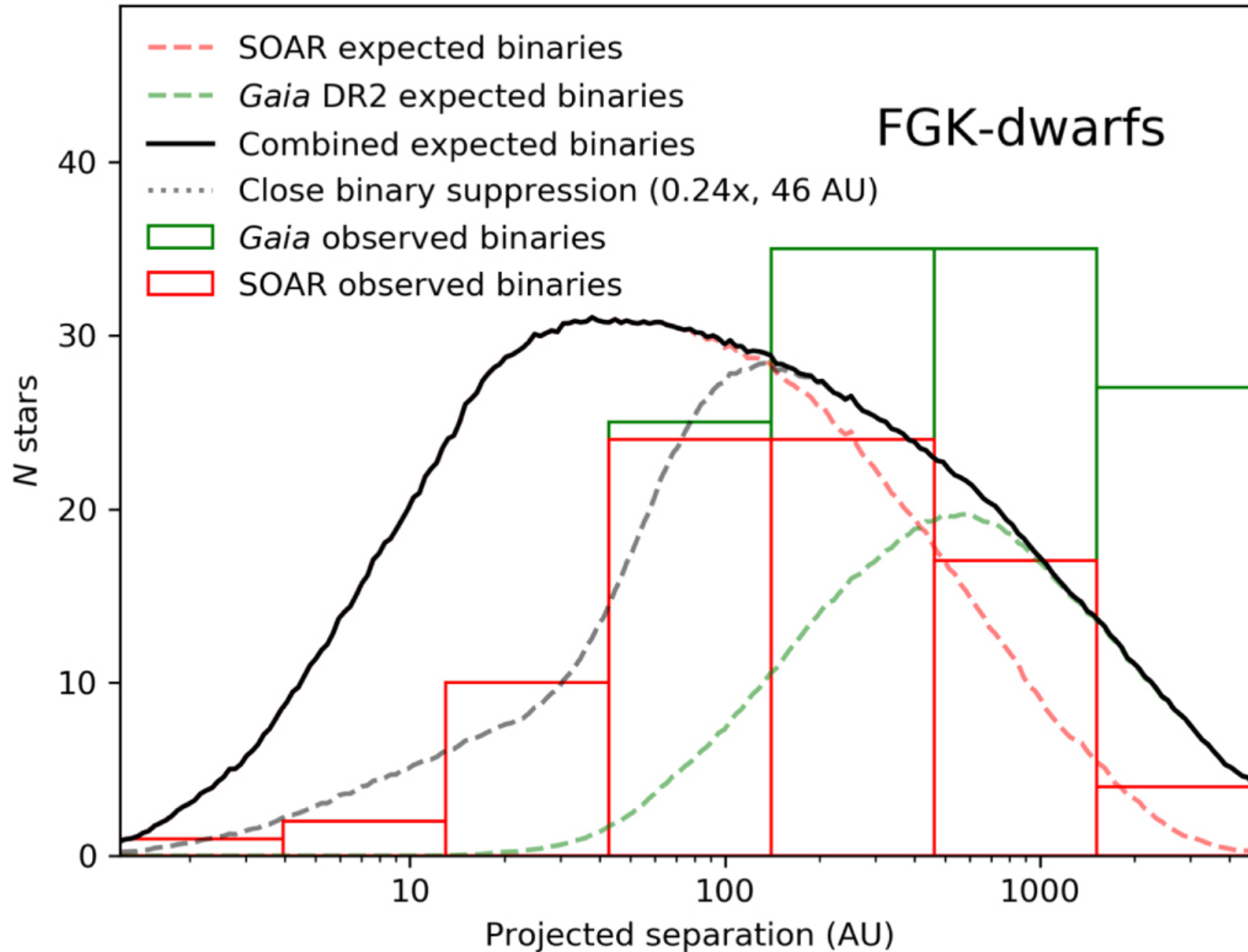
Figure 5. from SOAR TESS Survey. I. Sculpting of TESS Planetary Systems by Stellar Companions null 2020 AJ 159 19 doi:10.3847/1538-3881/ab55e9 https://dx.doi.org/10.3847/1538-3881/ab55e9 © 2019. The American Astronomical Society. All rights reserved.
