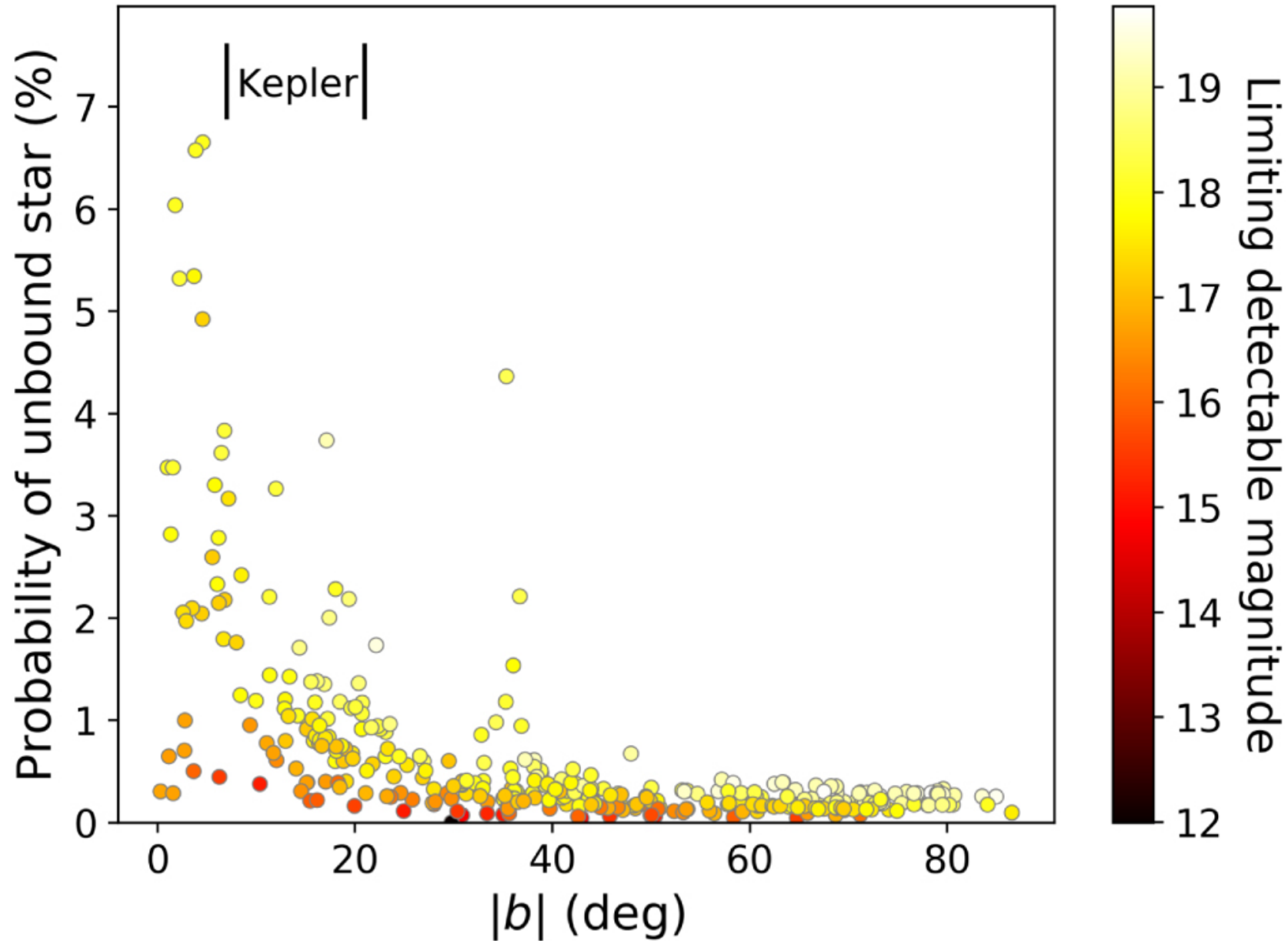
Figure 3. from SOAR TESS Survey. I. Sculpting of TESS Planetary Systems by Stellar Companions null 2020 AJ 159 19 doi:10.3847/1538-3881/ab55e9 https://dx.doi.org/10.3847/1538-3881/ab55e9 © 2019. The American Astronomical Society. All rights reserved.
