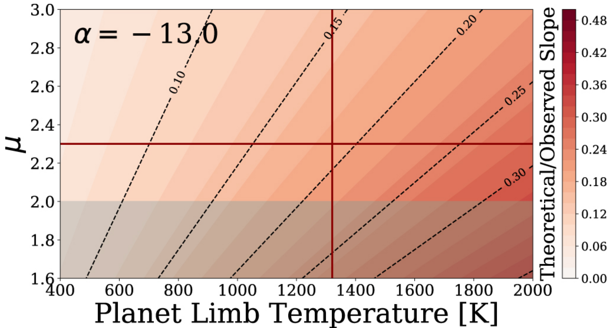
Figure 9. from MOPSS. II. Extreme Optical Scattering Slope for the Inflated Super-Neptune HATS-8b null 2020 AJ 159 7 doi:10.3847/1538-3881/ab5361 https://dx.doi.org/10.3847/1538-3881/ab5361 © 2019. The American Astronomical Society. All rights reserved.
