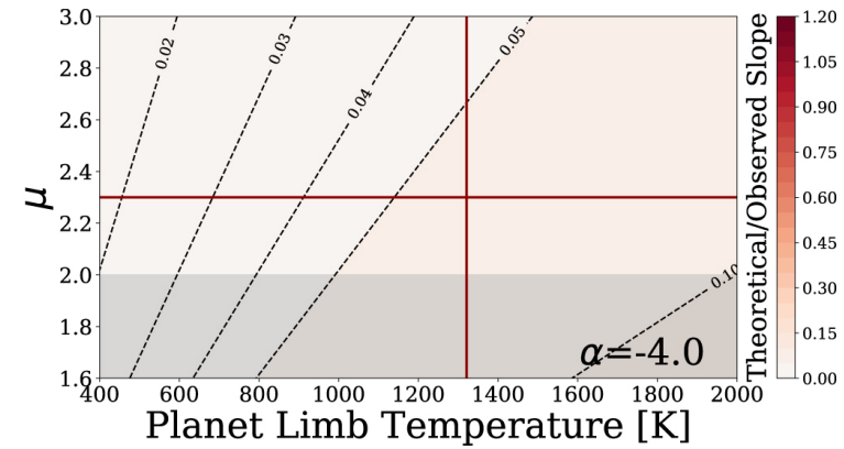
Figure 8. from MOPSS. II. Extreme Optical Scattering Slope for the Inflated Super-Neptune HATS-8b null 2020 AJ 159 7 doi:10.3847/1538-3881/ab5361 https://dx.doi.org/10.3847/1538-3881/ab5361
