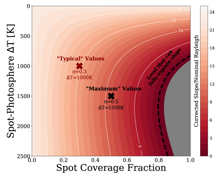
Figure 7. from MOPSS. II. Extreme Optical Scattering Slope for the Inflated Super-Neptune HATS-8b null 2020 AJ 159 7 doi:10.3847/1538-3881/ab5361 https://dx.doi.org/10.3847/1538-3881/ab5361 © 2019. The American Astronomical Society. All rights reserved.
