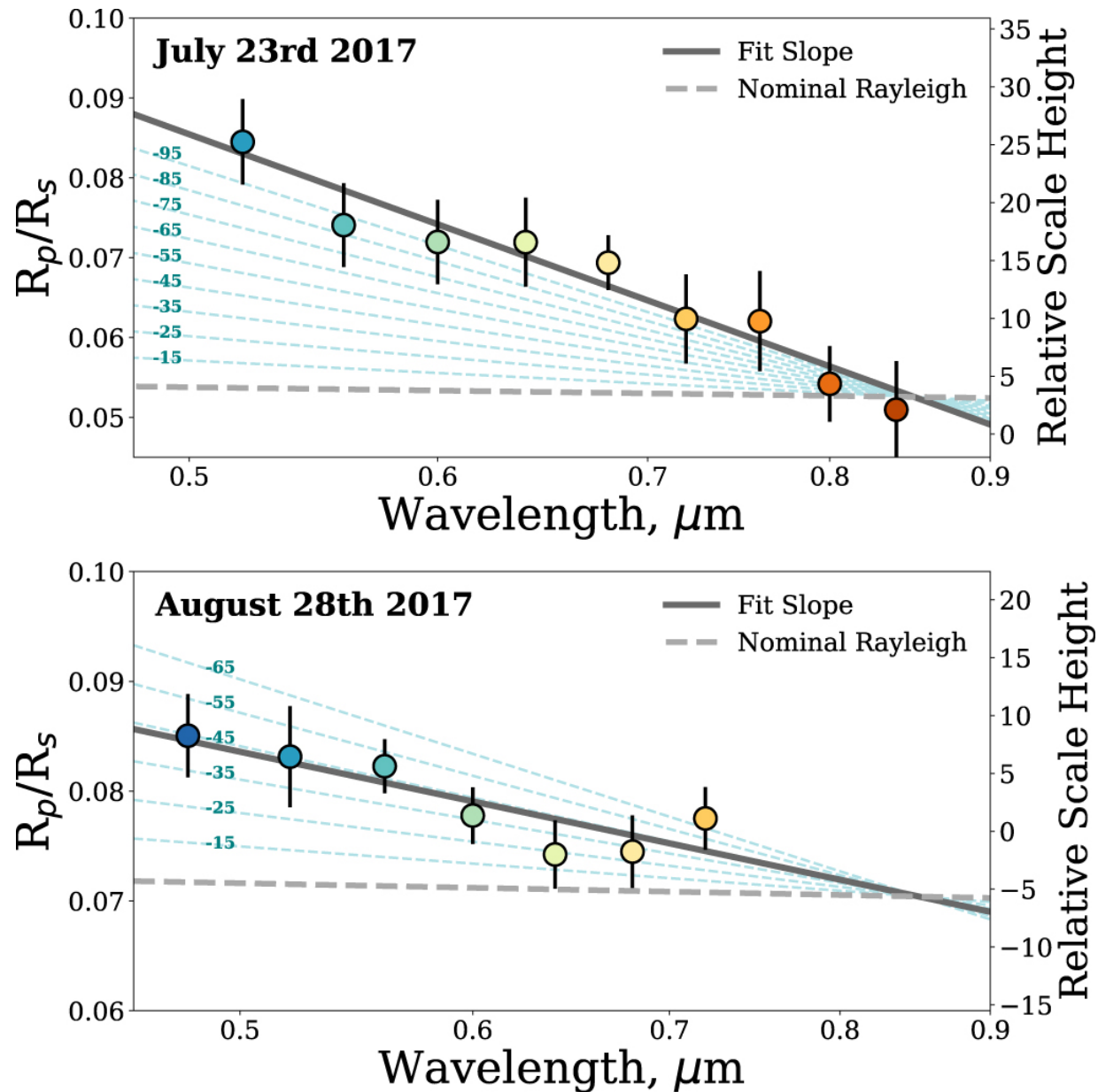
Figure 6. from MOPSS. II. Extreme Optical Scattering Slope for the Inflated Super-Neptune HATS-8b null 2020 AJ 159 7 doi:10.3847/1538-3881/ab5361 https://dx.doi.org/10.3847/1538-3881/ab5361
