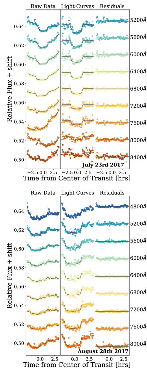
Figure 4. from MOPSS. II. Extreme Optical Scattering Slope for the Inflated Super-Neptune HATS-8b null 2020 AJ 159 7 doi:10.3847/1538-3881/ab5361 https://dx.doi.org/10.3847/1538-3881/ab5361 © 2019. The American Astronomical Society. All rights reserved.
