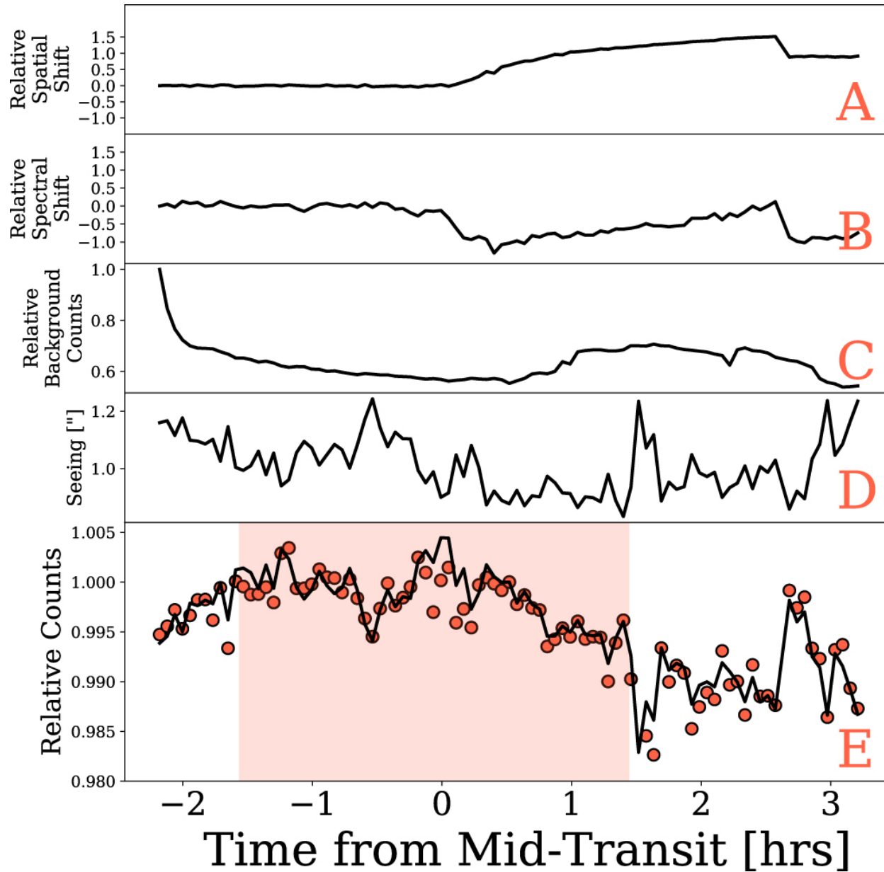
Figure 3. from MOPSS. II. Extreme Optical Scattering Slope for the Inflated Super-Neptune HATS-8b null 2020 AJ 159 7 doi:10.3847/1538-3881/ab5361 https://dx.doi.org/10.3847/1538-3881/ab5361 © 2019. The American Astronomical Society. All rights reserved.
