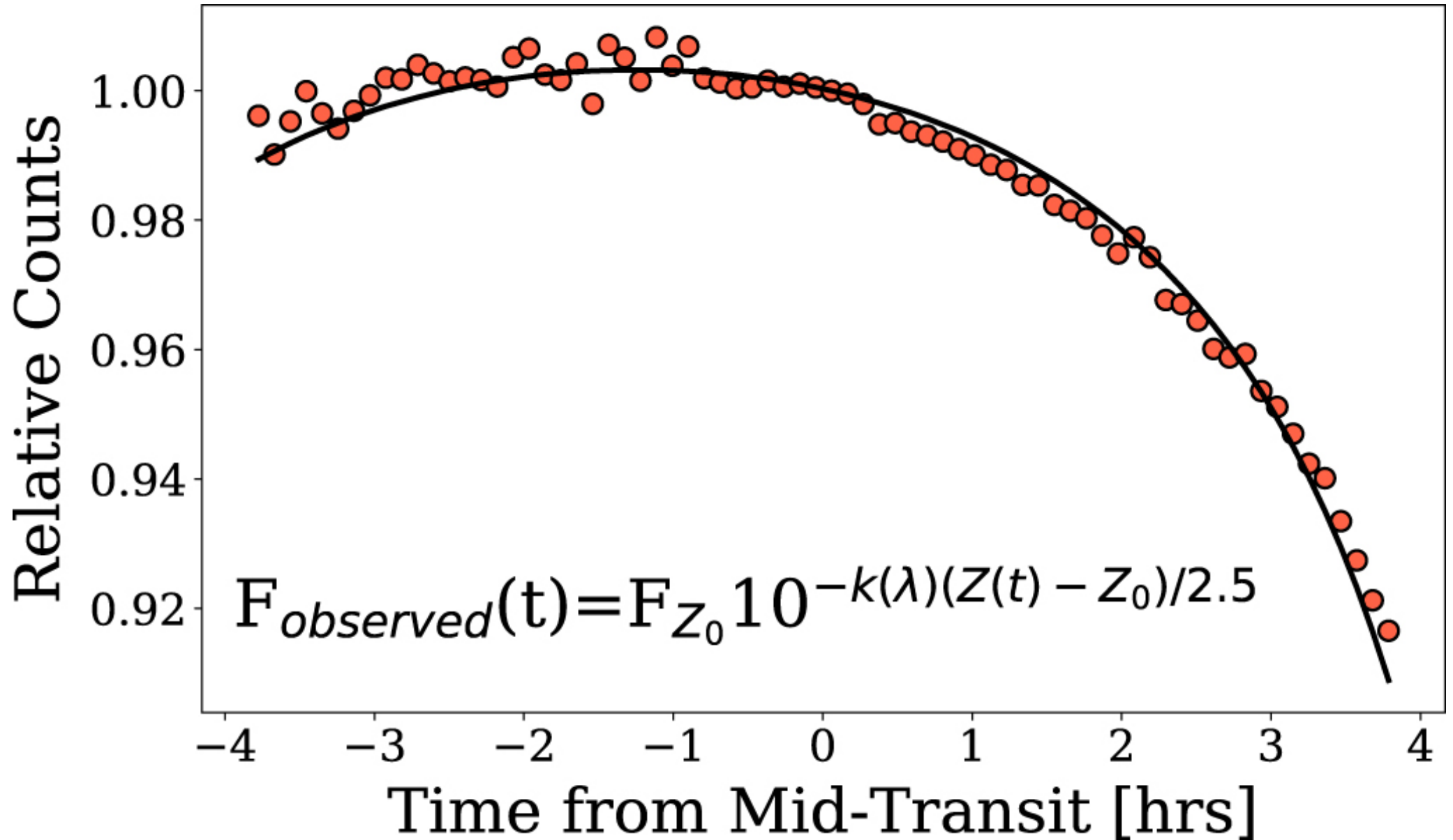
Figure 2. from MOPSS. II. Extreme Optical Scattering Slope for the Inflated Super-Neptune HATS-8b null 2020 AJ 159 7 doi:10.3847/1538-3881/ab5361 https://dx.doi.org/10.3847/1538-3881/ab5361 © 2019. The American Astronomical Society. All rights reserved.
