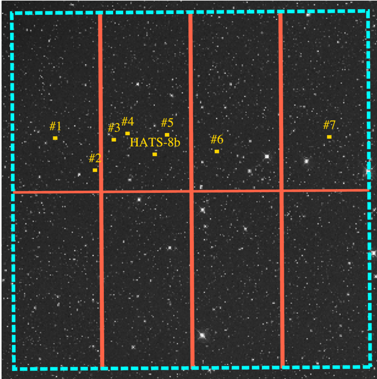
Figure 1. from MOPSS. II. Extreme Optical Scattering Slope for the Inflated Super-Neptune HATS-8b null 2020 AJ 159 7 doi:10.3847/1538-3881/ab5361 https://dx.doi.org/10.3847/1538-3881/ab5361 © 2019. The American Astronomical Society. All rights reserved.
