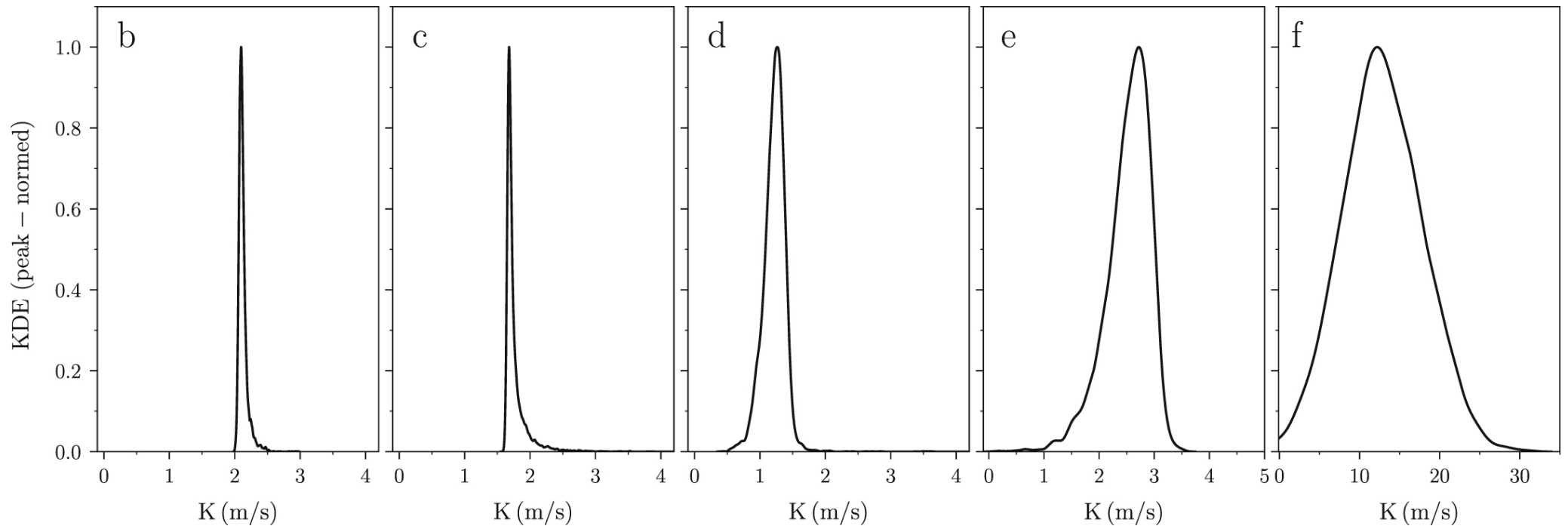
Figure 8. from Asteroseismology of the Multiplanet System K2-93 null 2019 AJ 158 248 doi:10.3847/1538-3881/ab5280 https://dx.doi.org/10.3847/1538-3881/ab5280 © 2019. The American Astronomical Society. All rights reserved.
