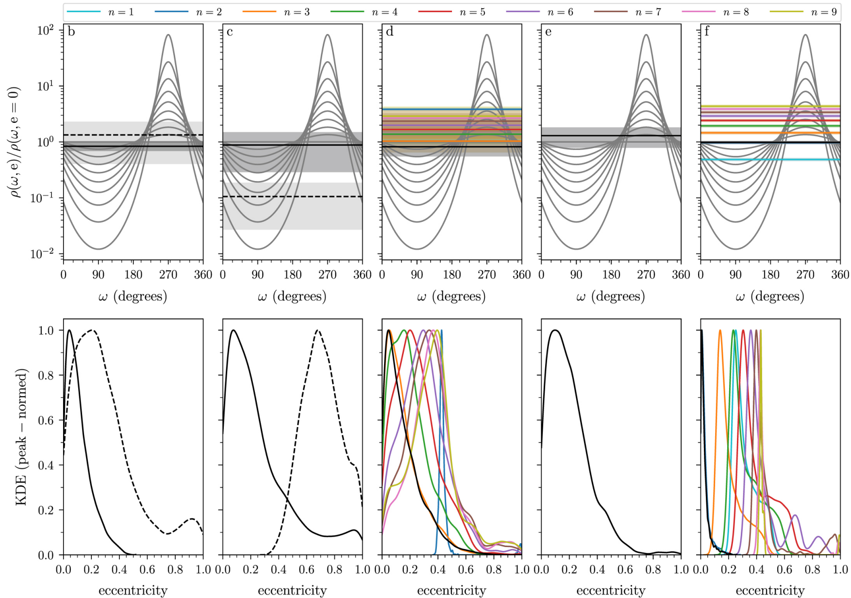
Figure 7. from Asteroseismology of the Multiplanet System K2-93 null 2019 AJ 158 248 doi:10.3847/1538-3881/ab5280 https://dx.doi.org/10.3847/1538-3881/ab5280 © 2019. The American Astronomical Society. All rights reserved.
