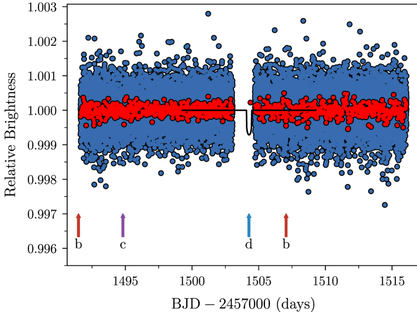
Figure 6. from Asteroseismology of the Multiplanet System K2-93 null 2019 AJ 158 248 doi:10.3847/1538-3881/ab5280 https://dx.doi.org/10.3847/1538-3881/ab5280 © 2019. The American Astronomical Society. All rights reserved.
