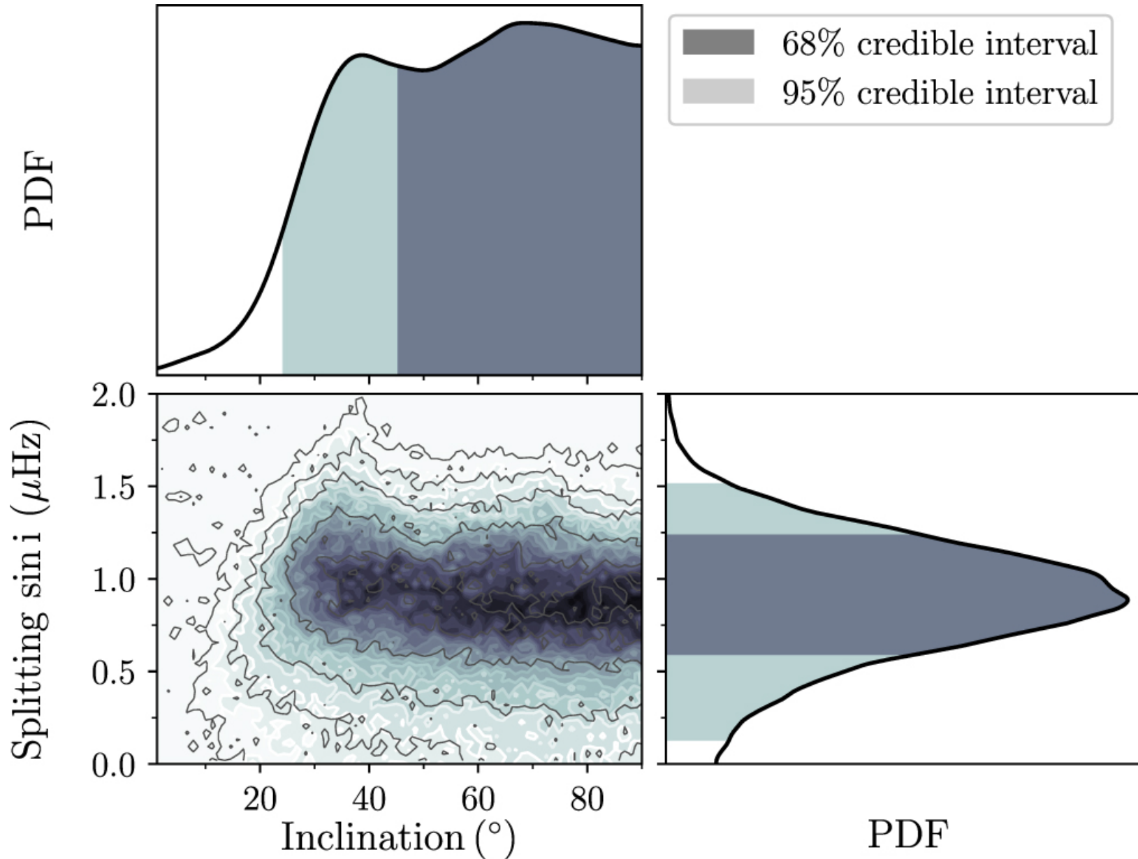
Figure 3. from Asteroseismology of the Multiplanet System K2-93 null 2019 AJ 158 248 doi:10.3847/1538-3881/ab5280 https://dx.doi.org/10.3847/1538-3881/ab5280 © 2019. The American Astronomical Society. All rights reserved.
