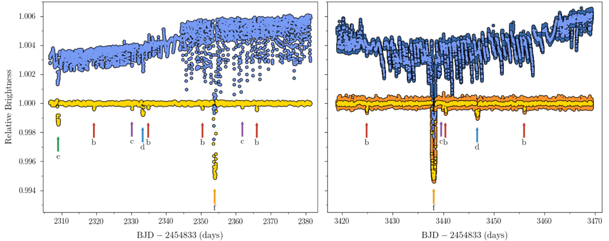
Figure 1. from Asteroseismology of the Multiplanet System K2-93 null 2019 AJ 158 248 doi:10.3847/1538-3881/ab5280 https://dx.doi.org/10.3847/1538-3881/ab5280 © 2019. The American Astronomical Society. All rights reserved.
